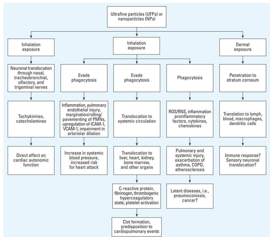
Figure 3. Hypothetical schema of potential interactions that may occur via inhalation of UFPs and translocation to other organs. Abbreviations: ICAM-1, intracellular adhesion molecule-1; PMNs, polymorphonuclear leukocytes; RNS, reactive nitrogen species; VCAM-1, vascular adhesion molecule-1. Schema also shows suspected interactions (indicated by a question mark) leading to sequences of events that may cause cardiovascular and pulmonary morbidity and mortality.
