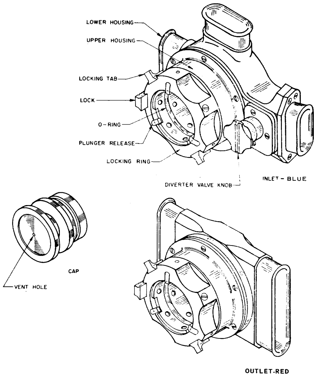
Figure I-23. - Gas connectors.
