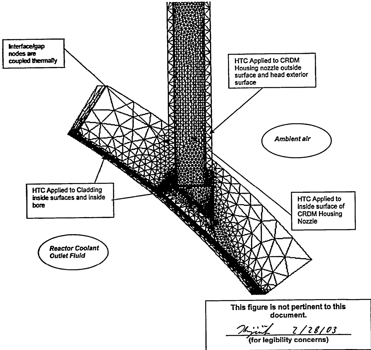
Figure 2 Heat Transfer Regions of Thermal Analysis Model
