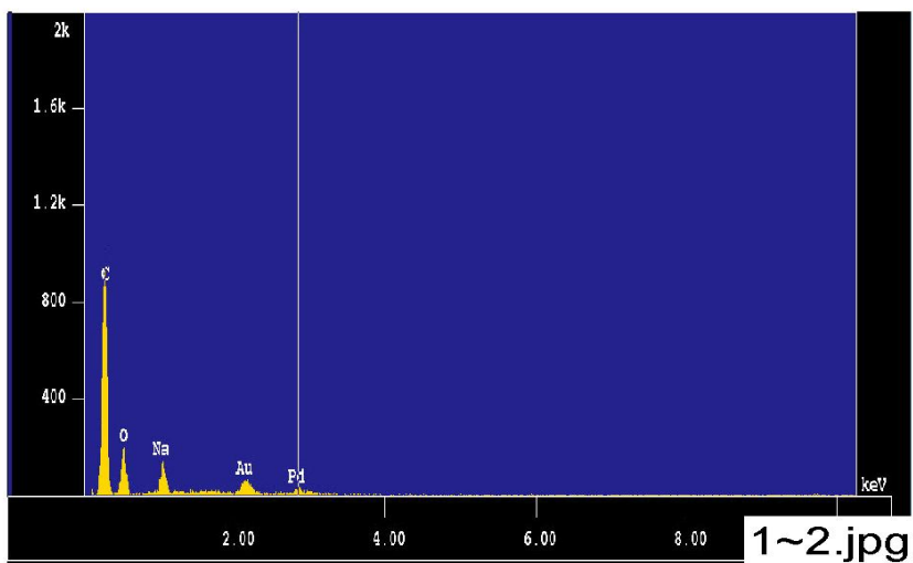
Figure B-4. Day-15, sample #1 counting spectrum (EDS 1-2) for the surface on the film overlying the filter (see Figure B-2).
