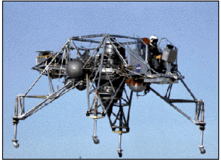
Lunar Landing Research Vehicle in flight. NASA photo EC64 506
