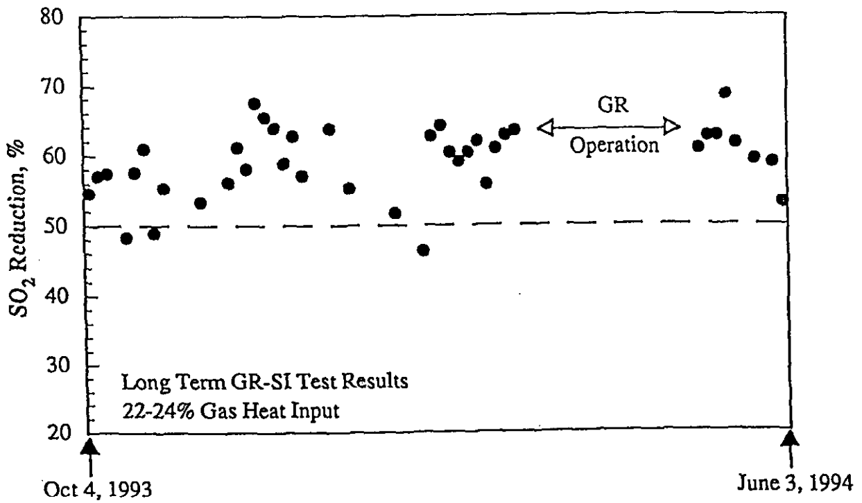
Figure 5-25b. Long term testing SO 2 emissions reduction
