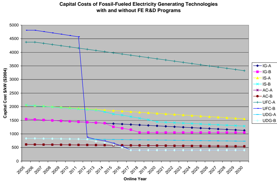
Figure 4. NEMS EMM Input Assumptions for Power Systems Program Capital Costs
