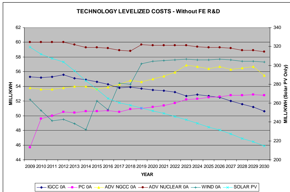
Figure 8. Levelized Costs Without FE R&D
