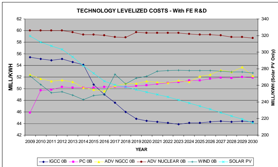
Figure 9. Levelized Costs With FE R&D
