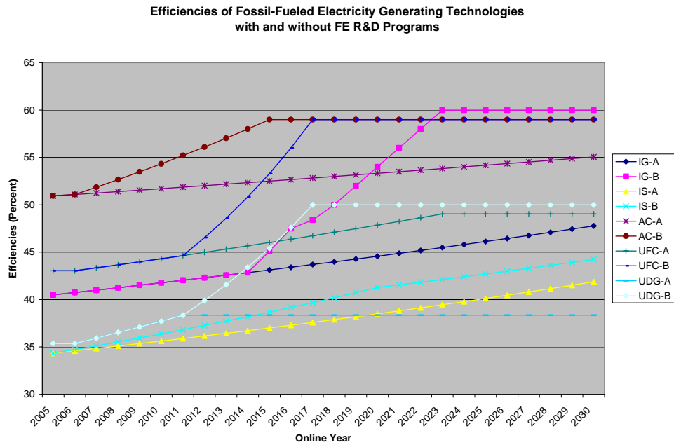
Figure 5. NEMS EMM Input Assumptions for Power Systems Program Efficiencies
