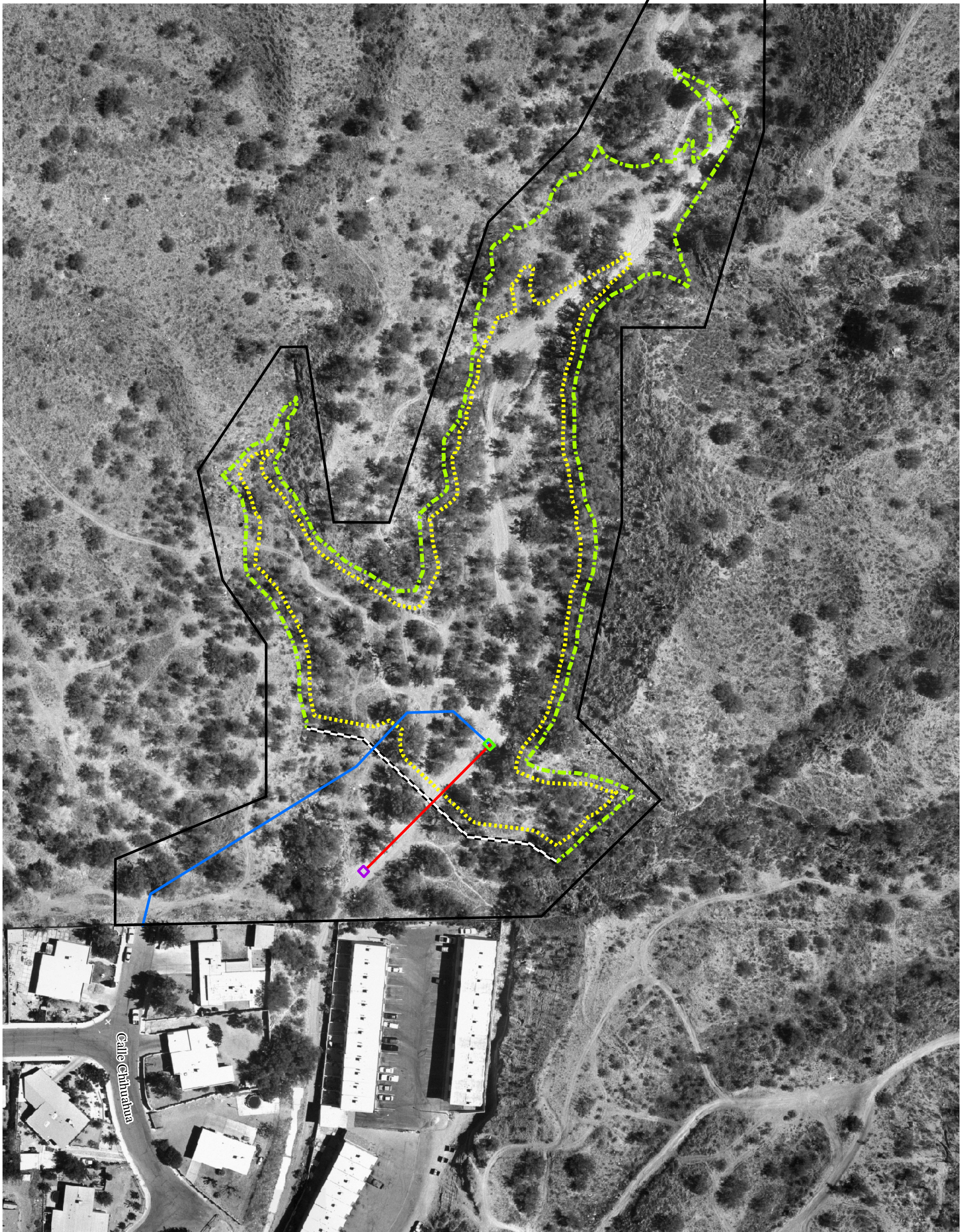
Figure 4 Chihuahua Wash Storm Water Detention/Sedimentation Basin
