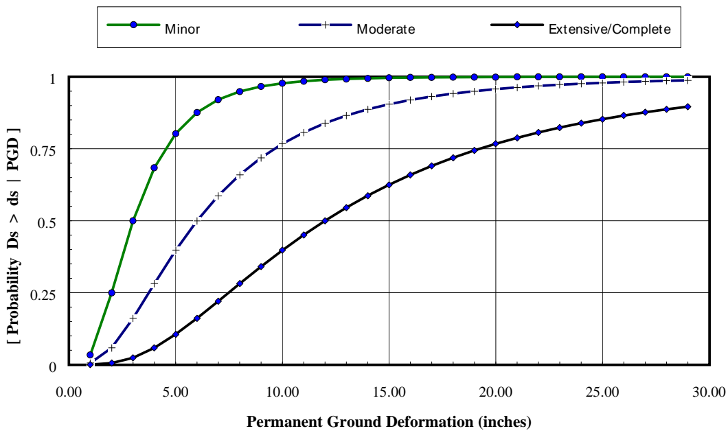
Figure 7.27 Fragility Curves for Stationary Cranes/Cargo Handling Equipment Subject to Permanent Ground Deformation.
