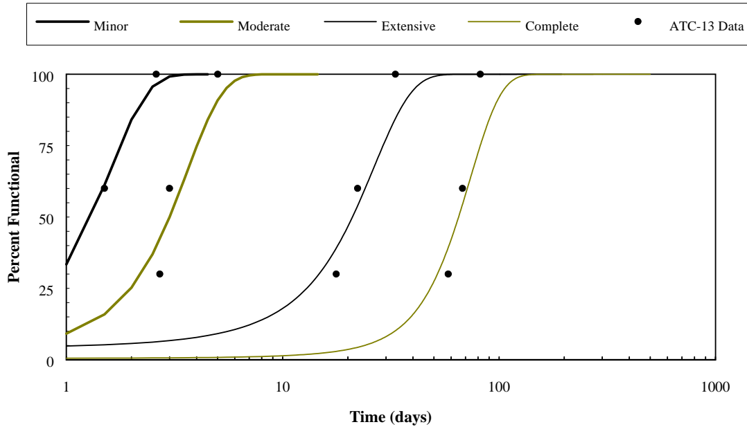
Figure 8.24: Restoration Curves for Lift Stations.
