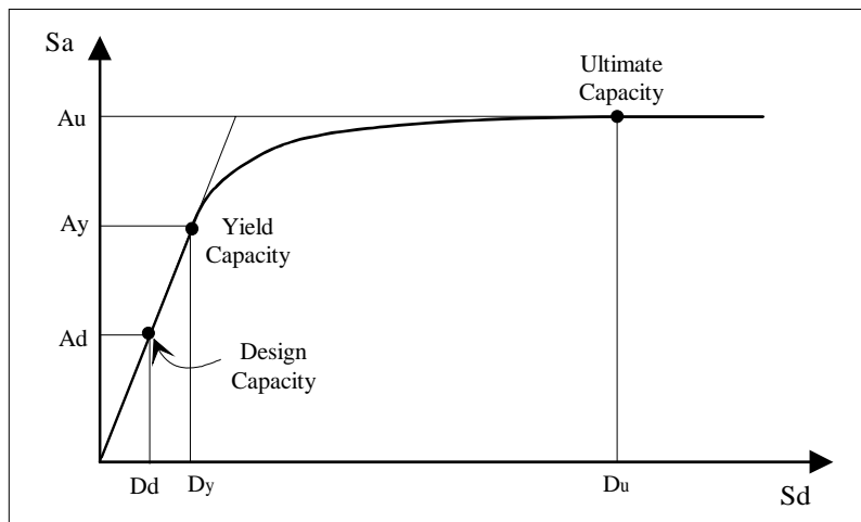
Figure 6.3 Example Building Capacity Curve.
