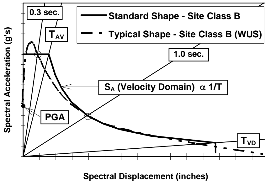
Figure 4.2 Standardized Response Spectrum Shape
