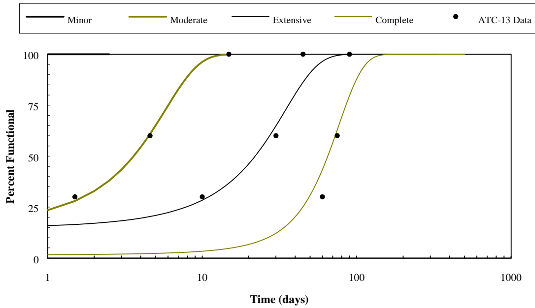
Figure 8.45: Restoration Curves for Generation Facilities.
