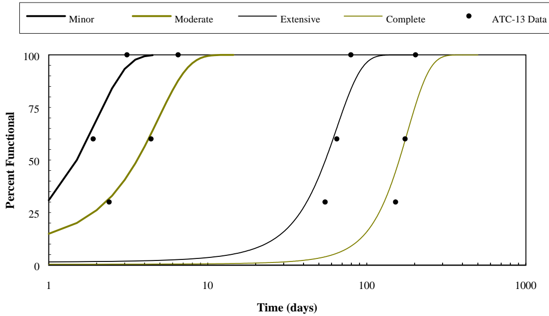
Figure 8.25: Restoration Curves for Waste Water Treatment Plants.
