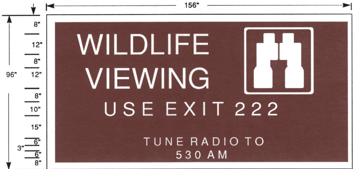
ITEM A (From a design by Colorado Department of Highways) Logo: 24" X 24"
