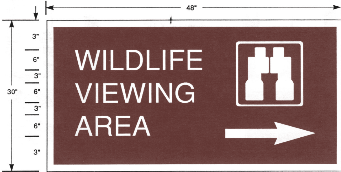
ITEM B Logo: 18" X 18" Arrow: 6" X 24"
