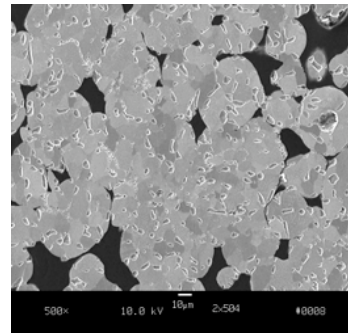
Figure 7. SEM images of sintered Ni-Cr-2xAl-Fe powder, 25 µm > dia. < 45 µm.
