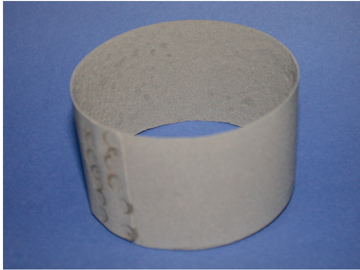
Figure 9. Resistance spot welded porous cylinder of sintered Ni-Cr-2xAl-Fe powder.
