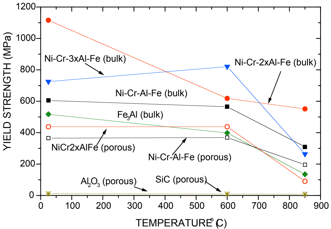
Figure 6. Yield strength results from asymmetric four point bend (AFPB) tests, performed at the indicated temperatures.
