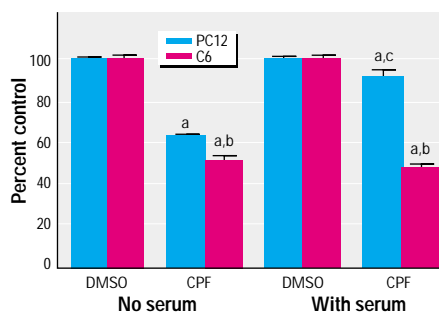
Figure 3. Effects of standard serum conditions on the ability of chlorpyrifos (CPF; 15 \mu M) to inhibit DNA synthesis in PC12 and C6 cells. PC12 cells were grown in the presence of 10% horse serum + 5% fetal bovine serum; C6 cells were grown with 5% fetal bovine serum. Serum was then deleted (no serum) or continued (with serum) during the chlorpyrifos exposure period. Data represent means and SEs obtained from 9–11 determinations for each treatment and cell type, presented as the percentage of corresponding control values: 13,600 \pm 120 dpm/ \mu g DNA for PC12 cells without serum, 10,700 \pm 150 with serum ( p < 0.0001 ); 6,600 \pm 100 for C6 cells without serum, 8,200 \pm 300 with serum ( p < 0.0002 ). DNA content was 27 \pm 1 \mu g/dish for PC12 cells and 33 \pm 1 for C6 cells, and was unaffected by the addition of serum or by the chlorpyrifos treatment (data not shown). ANOVA: treatment, p < 0.0001 ; treatment \times cell type, p < 0.0001 ; treatment \times serum, p < 0.0001 ; treatment \times cell type \times serum, p < 0.0001 . Treatment with chlorpyrifos elicited significant reductions in DNA synthesis (a) in both cell types in the absence of serum; the effect was greater on C6 than on PC12 cells (b). The addition of serum prevented most of the effect of chlorpyrifos on PC12 cells (c) but did not protect C6 cells.
