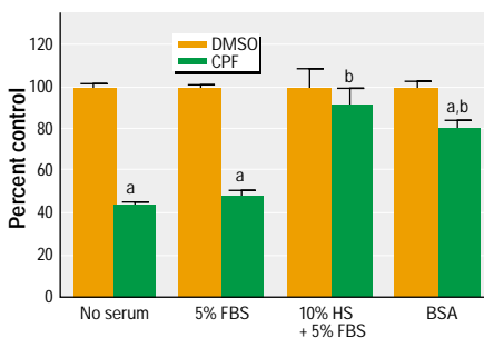
Figure 4. Effects of different serum mixtures on the ability of chlorpyrifos (15 \mu M) to inhibit DNA synthesis in C6 cells. C6 cells were grown with 5% fetal bovine serum (FBS) and then serum was either deleted or continued (no serum) during the chlorpyrifos exposure period, or a different serum mixture used for PC12 cells was added [10% horse serum (HS) + 5% FBS], or bovine serum albumin (BSA) was added to achieve the same protein concentration as in the PC12 serum mixture. Data represent means and standard errors obtained from 5–20 determinations for each combination of treatment and serum condition, presented as the percentage of corresponding control values (see legend to Figure 3). ANOVA: treatment, p < 0.0001 ; treatment \times serum, p < 0.0001 . Treatment with chlorpyrifos elicited significant reductions in DNA synthesis (a) in the presence or absence of 5% FBS. Addition of 10% HS + 5% FBS protected the cells from chlorpyrifos (b) and a similar protection was obtained with BSA.
