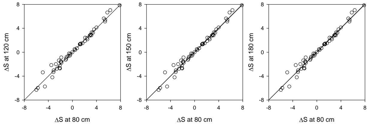
Figure 3-3. Relationships between changes of soil water storage in different soil layers for location BL1.
