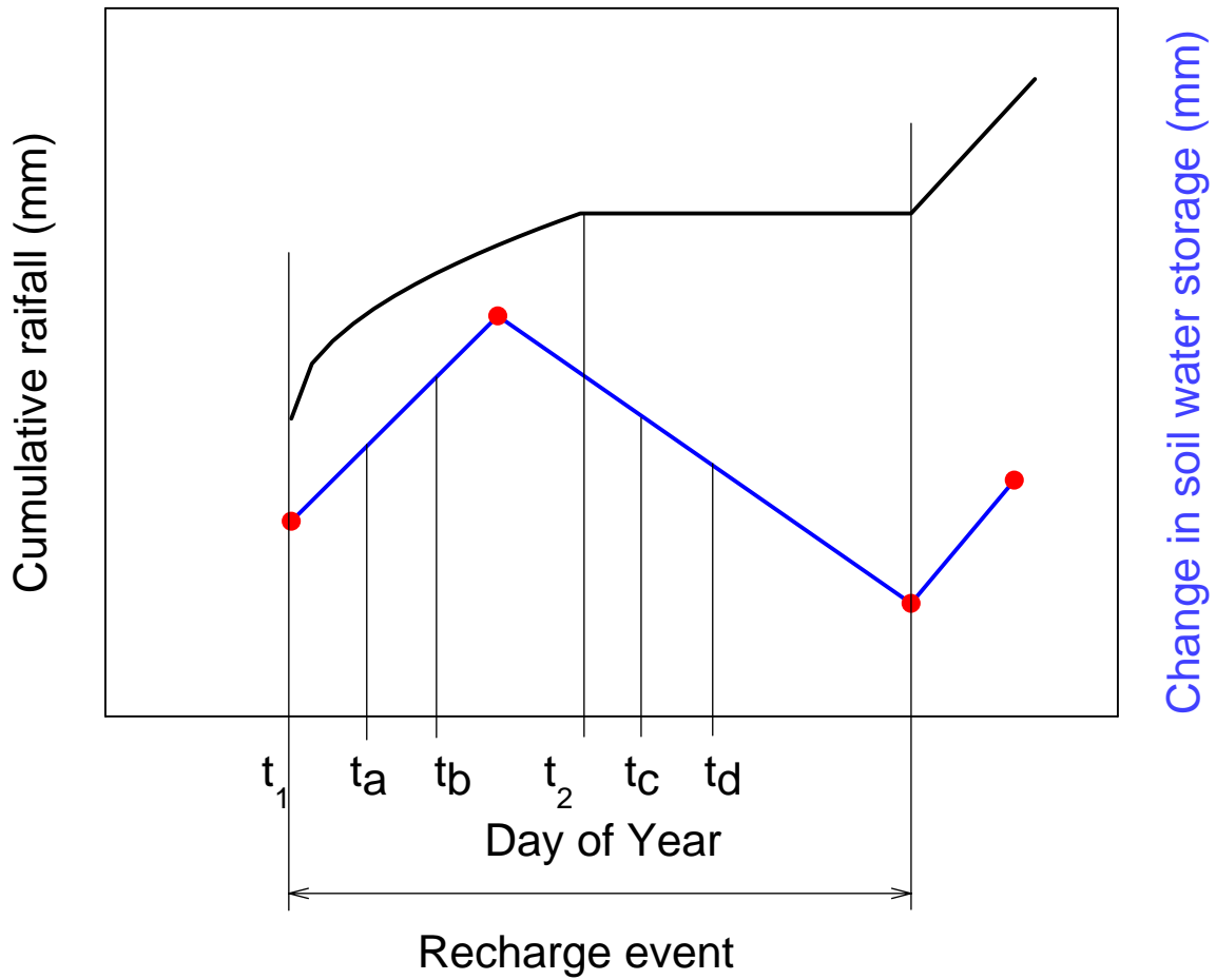
Figure 3-2. Schematics of the recharge event selection. Comments are in the text.
