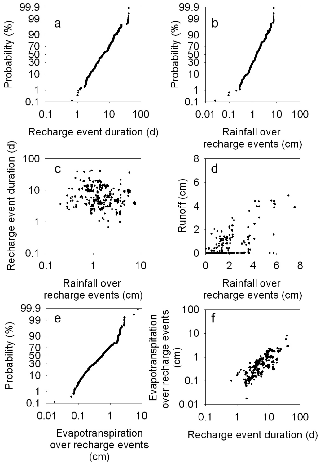
Figure 4-1. Statistics of soil water budget components integrated over recharge events.
