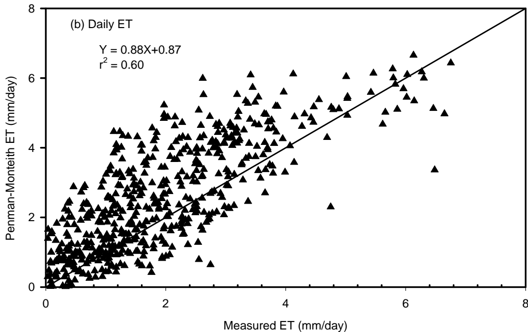
Figure 2-5. Comparison of evapotranspiration calculated using the FAO Penman-Monteith method and measured evapotranspiration using energy budget methods. Evapotranspiration was extrapolated (using solar radiation) for days that did not have measured data (May 1 - June 8, 2001 and January 1 - April 18, 2002).
