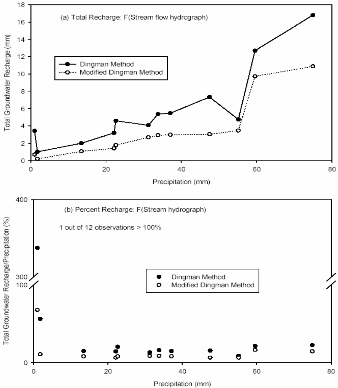
Figure 4-8. Ground-water recharge estimated with Dingman and Modified Dingman stream flow hydrograph separation methods. Twelve distinct stream flow hydrographs at station 3 were separated and analyzed in this study. Figure 4-8a shows total ground-water recharge versus precipitation, and Figure 4-8b shows ground-water recharge expressed as a percent of precipitation. High percent values were obtained at low rainfall events probably because of base flow from previous storms.
