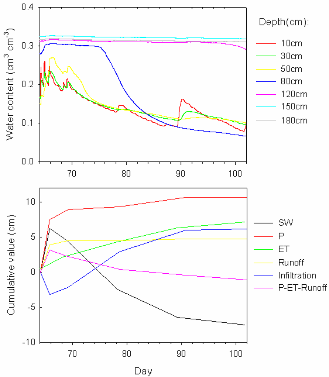
Figure 4-6. Soil water budget in presence of perched water.
