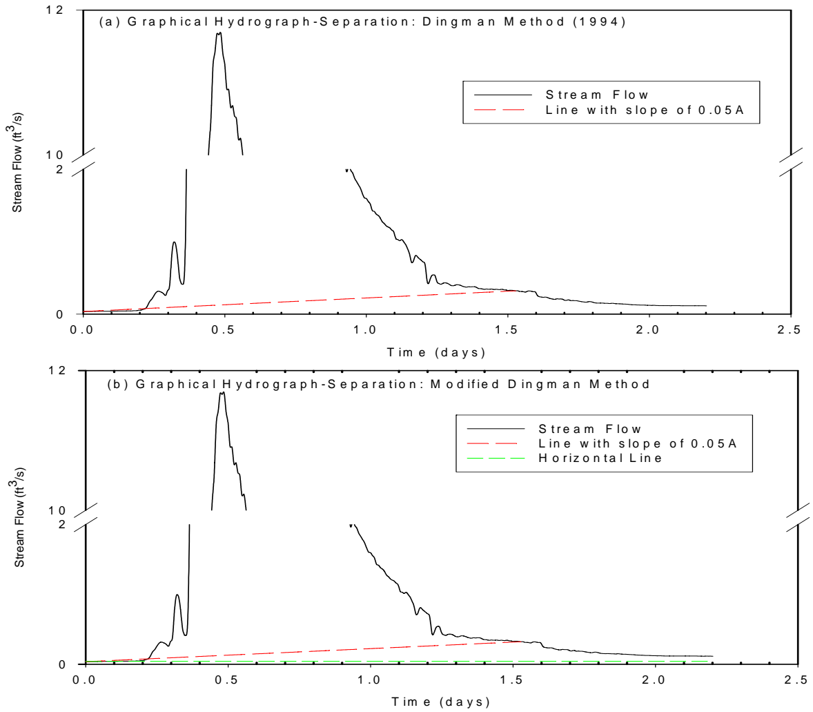
Figure C-1. Graphical stream flow hydrograph separation techniques
