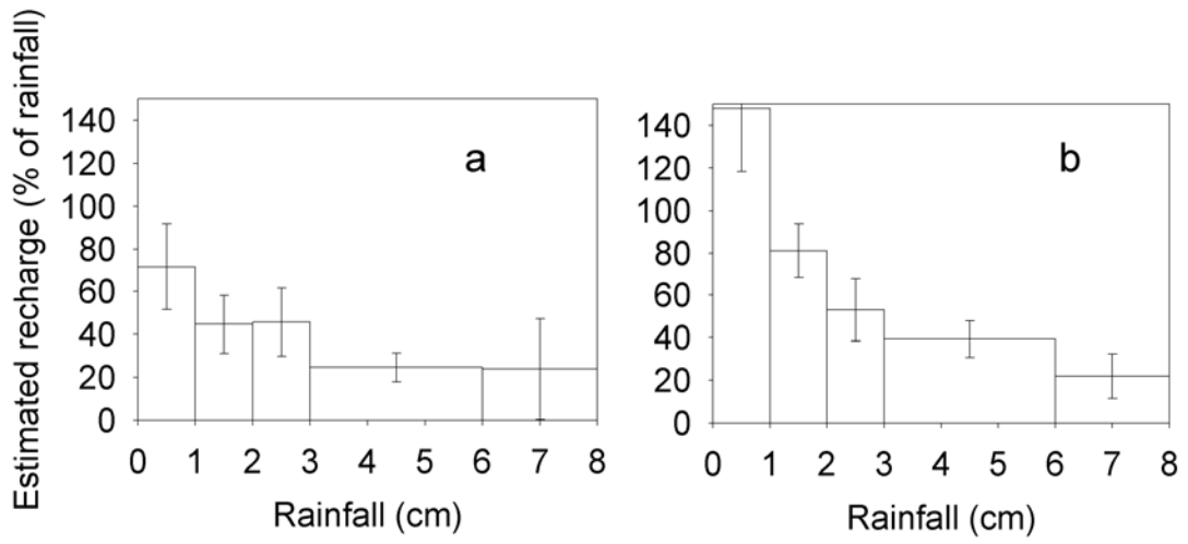
Figure 4-7. Fraction of precipitation used for recharge for different rainfall amounts at locations BL1, BL2, and BL3 (a) and at the rest of locations (b). Error bars show the standard error.
