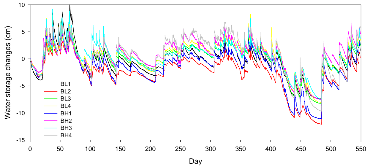
Figure 4-2. Changes in soil water storage in 0-80 cm soil layer during the period of observations.
