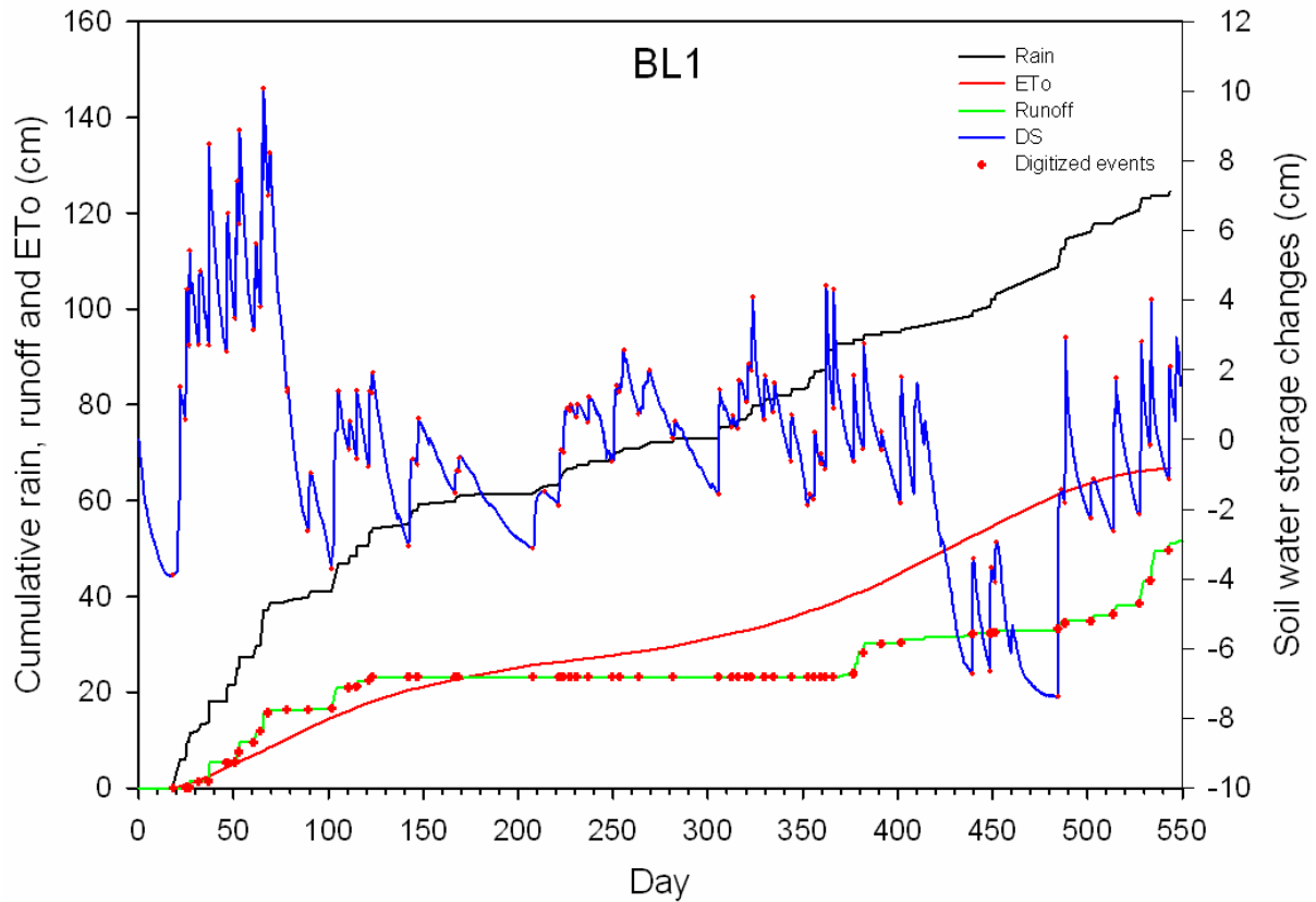
Figure 3-1. Selection of the recharge events from soil water storage time series at the location BL1. Dots mark minima and maxima on the soil water storage time series used to define recharge events.
