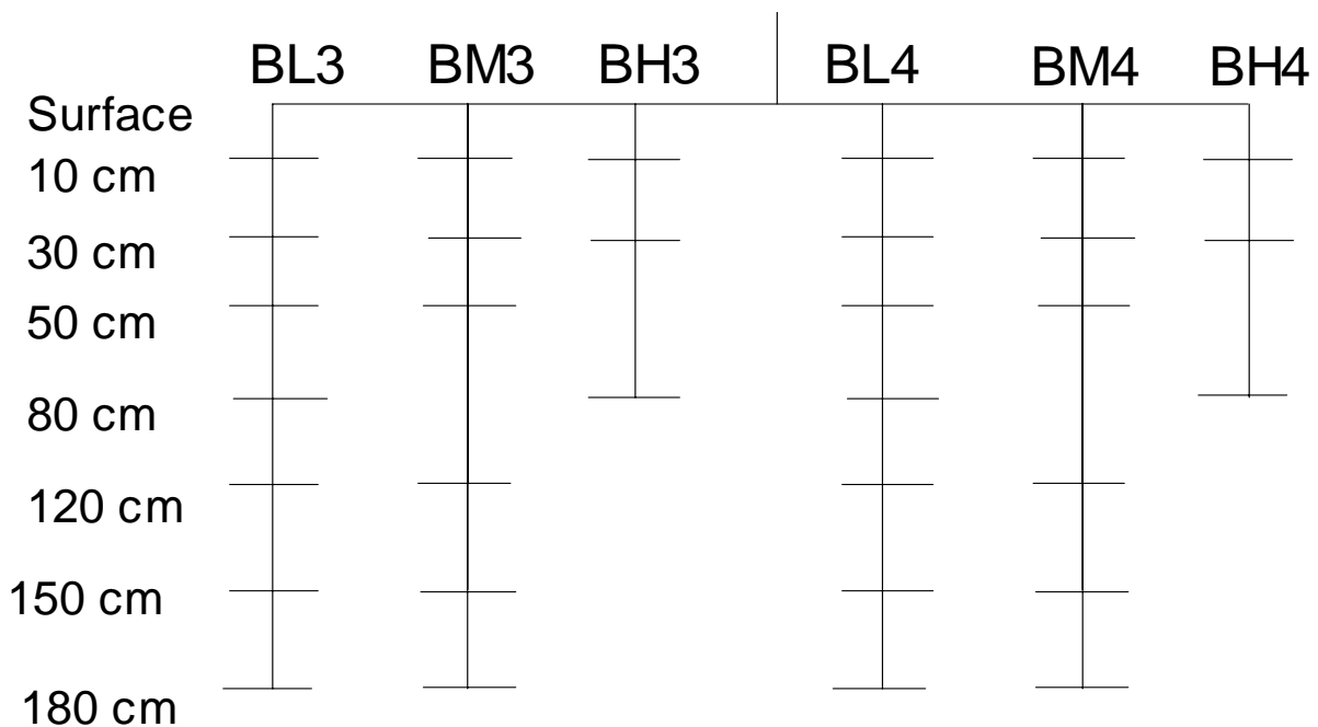
Figure 2-3. Installation depths of soil moisture sensors on a sample of 6 probes (out of 12) in the soil profile depending on the infiltration capacity of the probe location. Note that B refers to field B, L refers to probes installed in areas where infiltration capacity was high [low electromagnetic (EM) values]; M refers to probes installed in areas where infiltration capacity was medium (medium EM values); H refers to probes installed in areas where infiltration capacity was low (high EM values).
