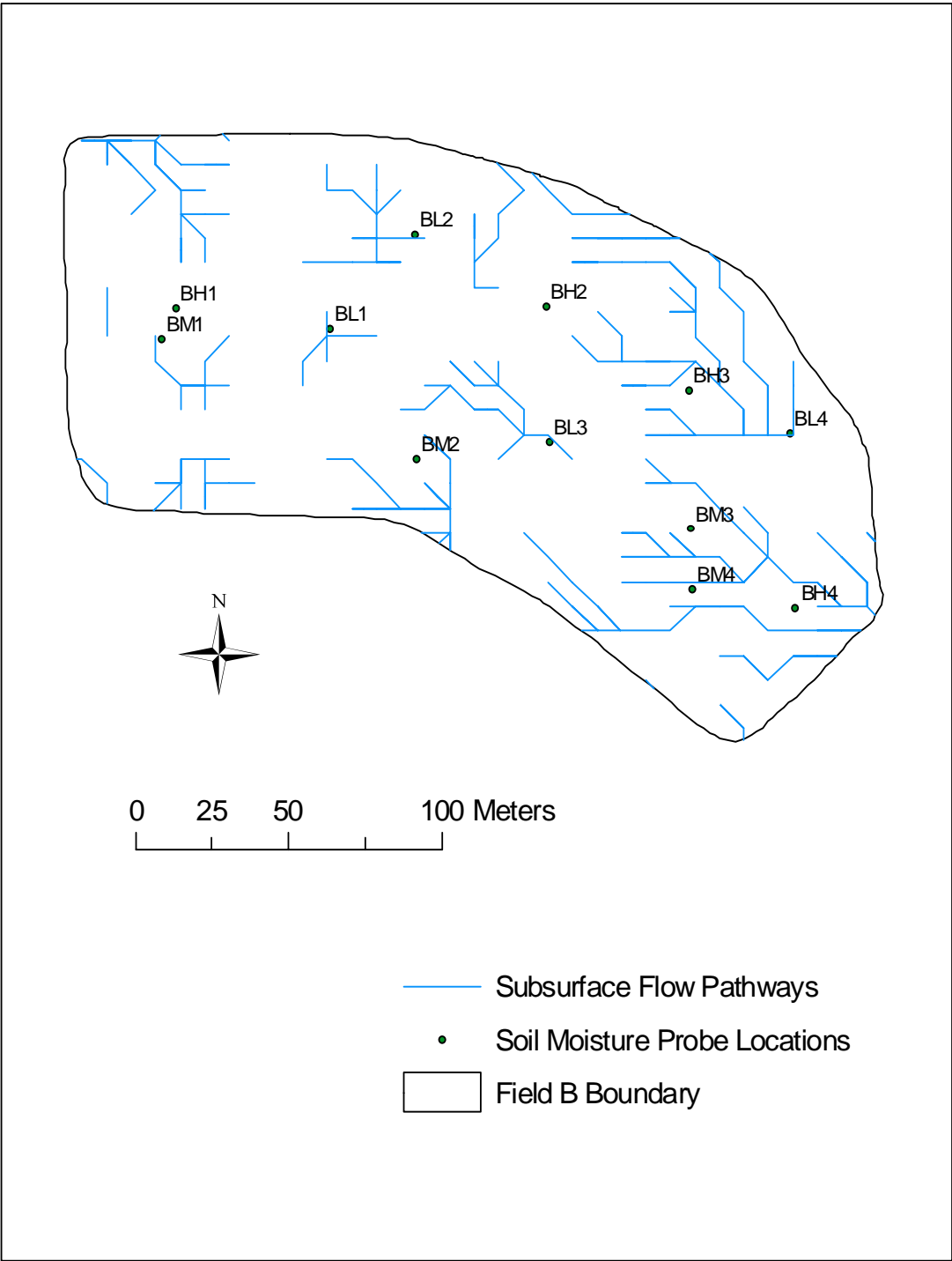
Figure 2-2. Subsurface flow pathways and locations of soil moisture multi-sensor capacitance probes (MCP) in field B.
