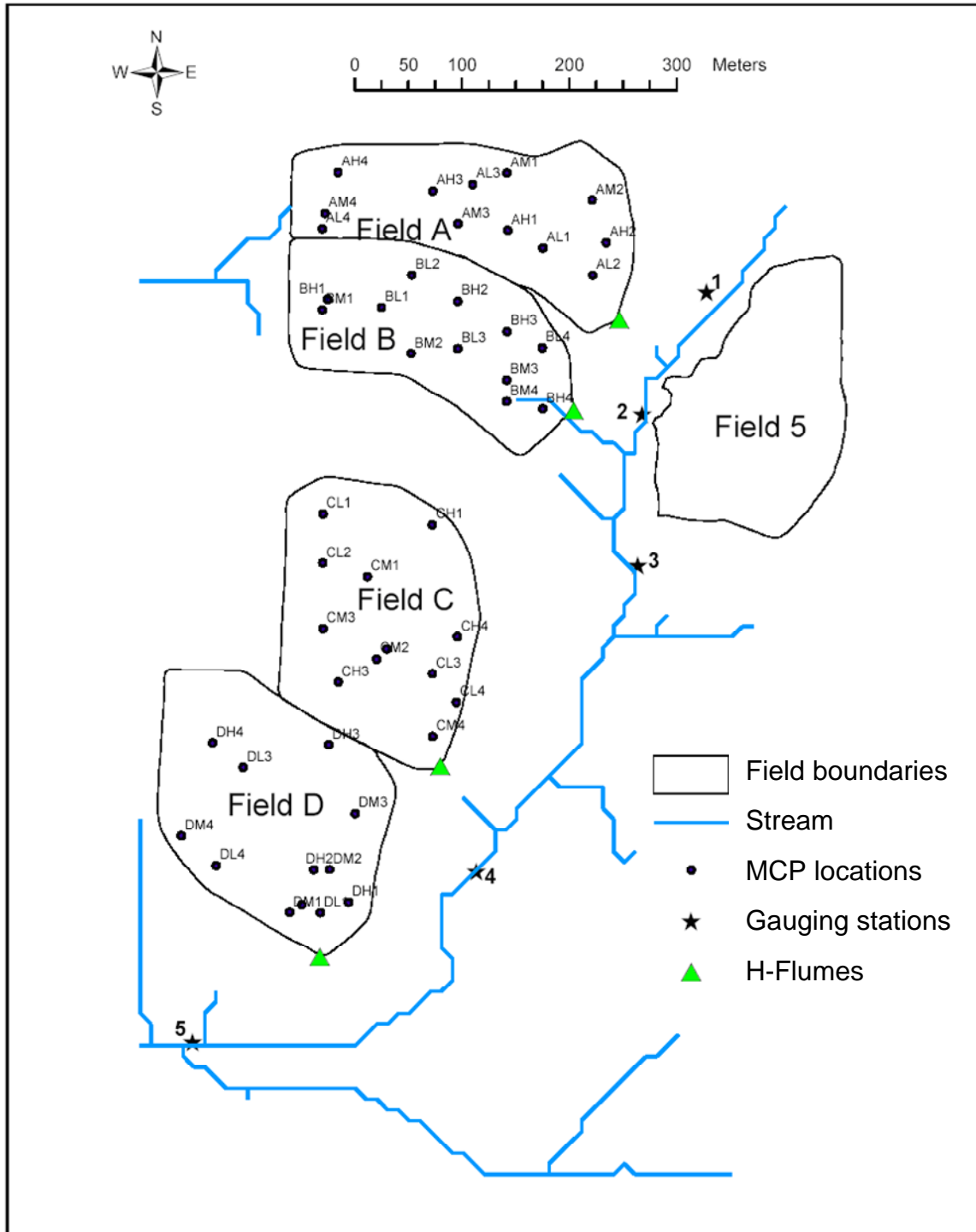
Figure 2-1. Layout of fields, soil moisture measuring probes, stream flow gauges, and surface runoff H-flumes at the research site. Note that L (as in AL, BL, or CL etc) refers to probes installed in areas where infiltration capacity was high [low electromagnetic (EM) values]; M refers to probes installed in areas where infiltration capacity was medium (medium EM values); H refers to probes installed in areas where infiltration capacity was low (high EM values). Only soil moisture data collected in field B were used in this study.
