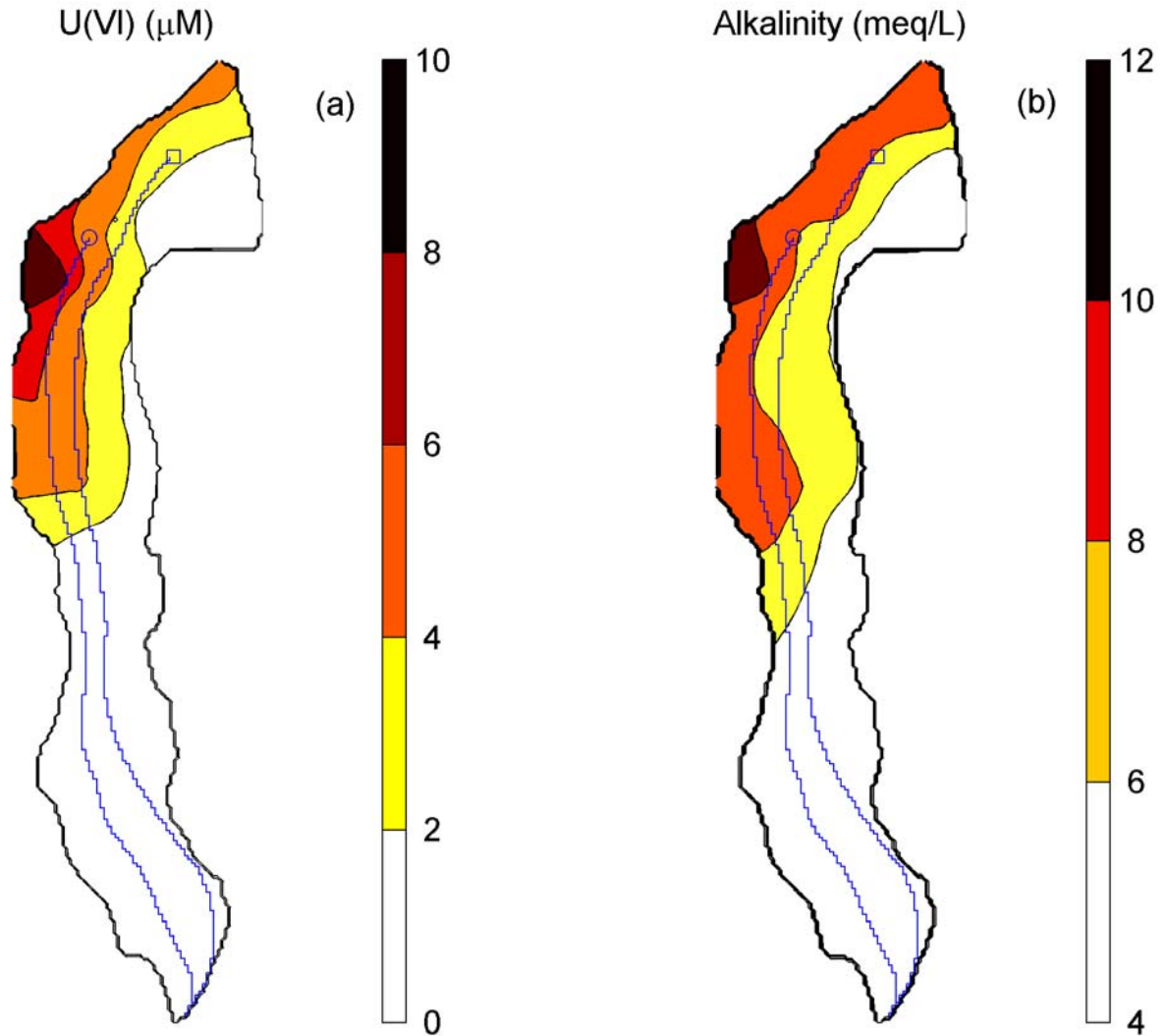
Figure 11.2. Existing distribution of U(VI) concentration and alkalinity in the Naturita alluvial aquifer. Also shown are the locations of the onsite well (□), the offsite well (○), and the groundwater flow path backtracked from the two wells.
