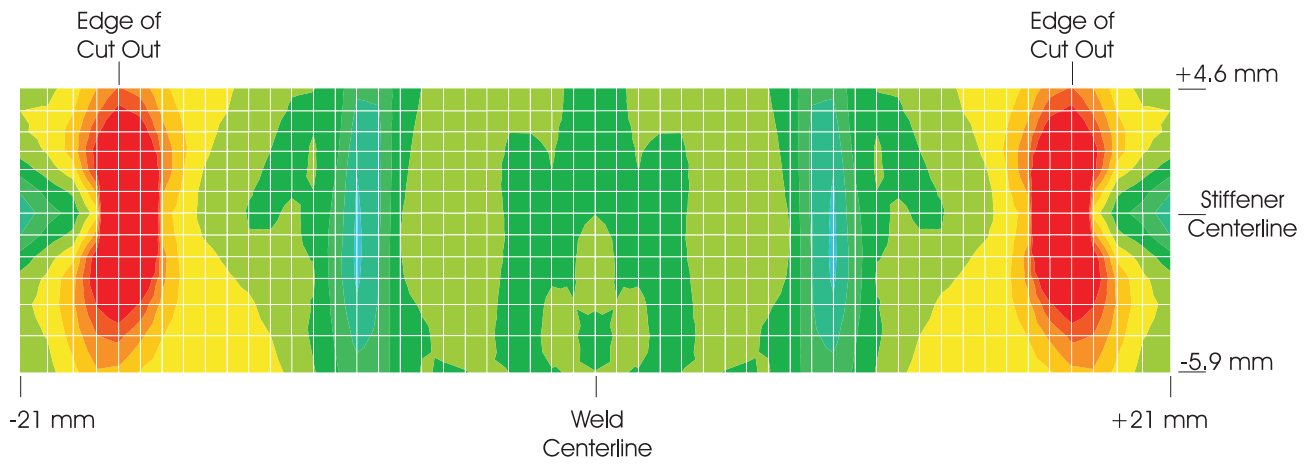
Enlarged Region Of Liner At Rathole Stiffener Cut Out
