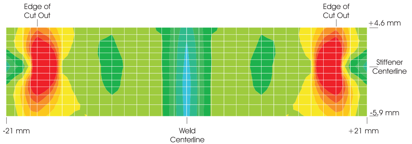
Figure 8-11. PCCV Liner Model 2, Posttest Analysis, Mesh Sensivity, Coarse Mesh, Horizontal Strain Contour Plot At End of Analysis (1.3 MPa)
