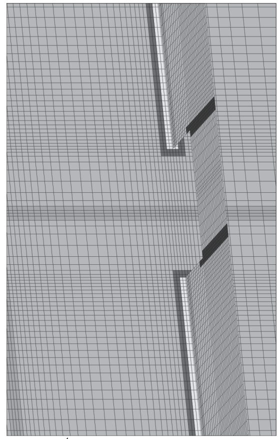
Figure 8-3. Liner Seam Model Geometric Details
