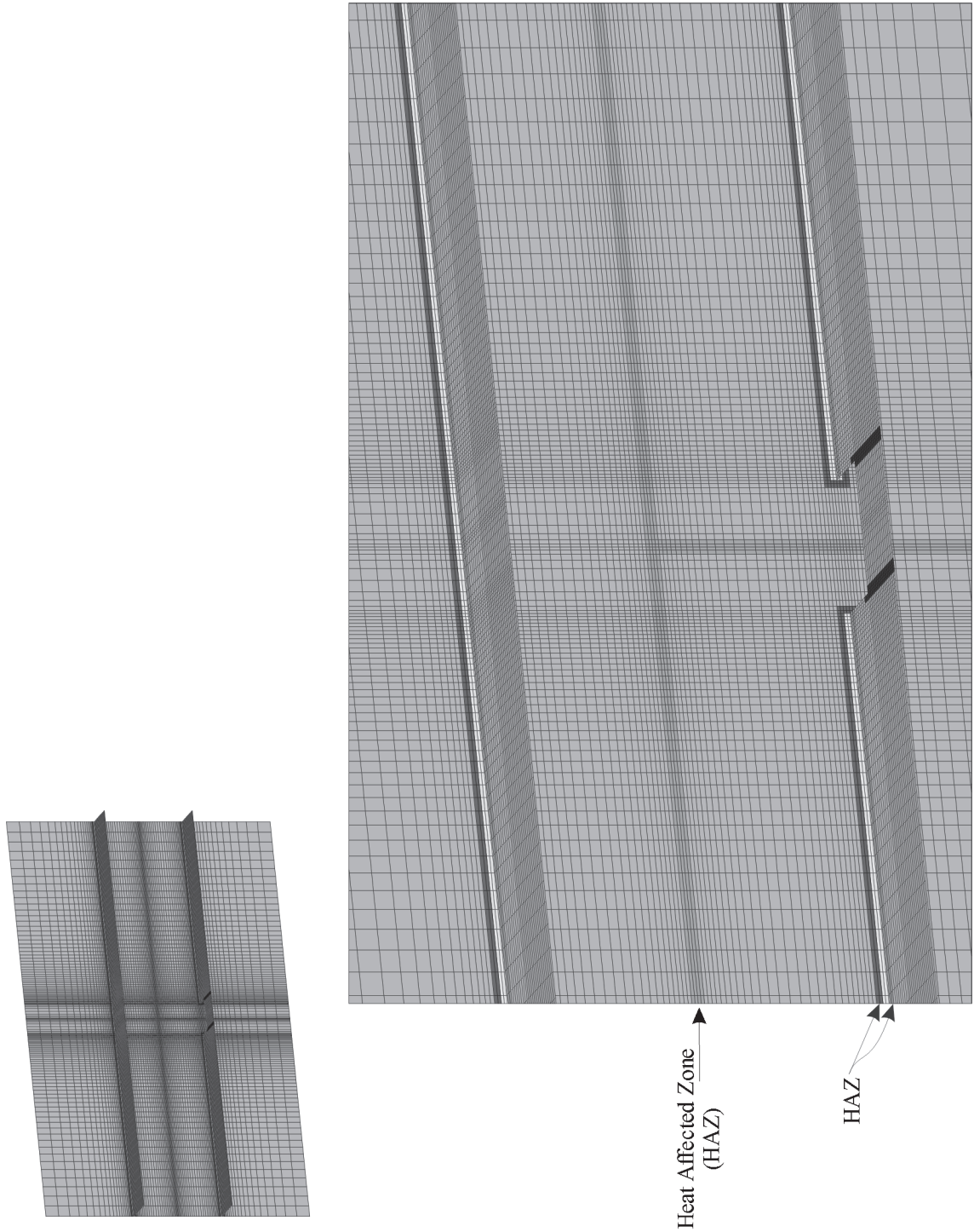
Figure 8-4. Liner Seam Model
