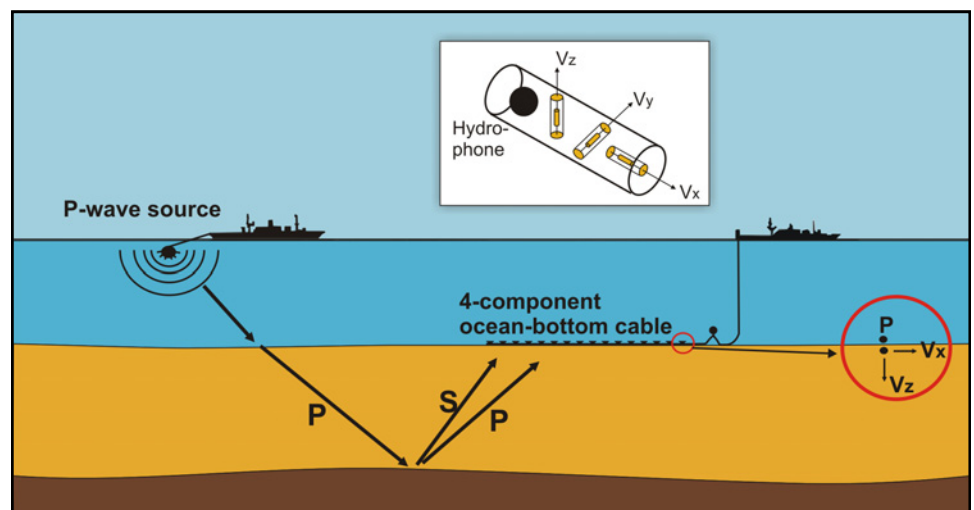
Acquisition principle for marine multi-component seismic data. The rays illustrate how a downgoing P-wave generates an upgoing P-wave, but also converts upon reflection, creating an upgoing S-wave.
