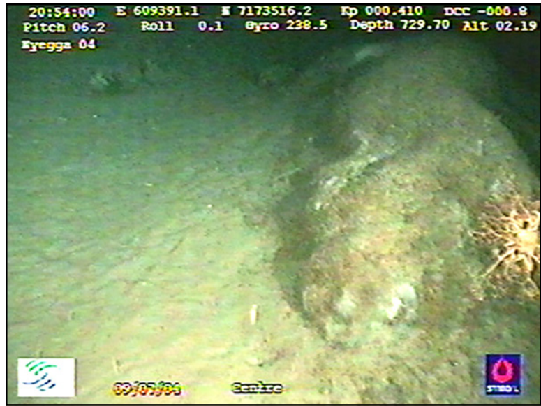
Second example of pingo-like feature found at G11 pockmark.
