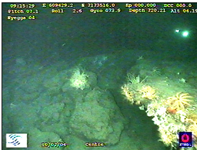
ROV photo taken inside the G11 complex pockmark showing terrain with large carbonate rocks (lights at upper right from second ROV at 15 m distance).
