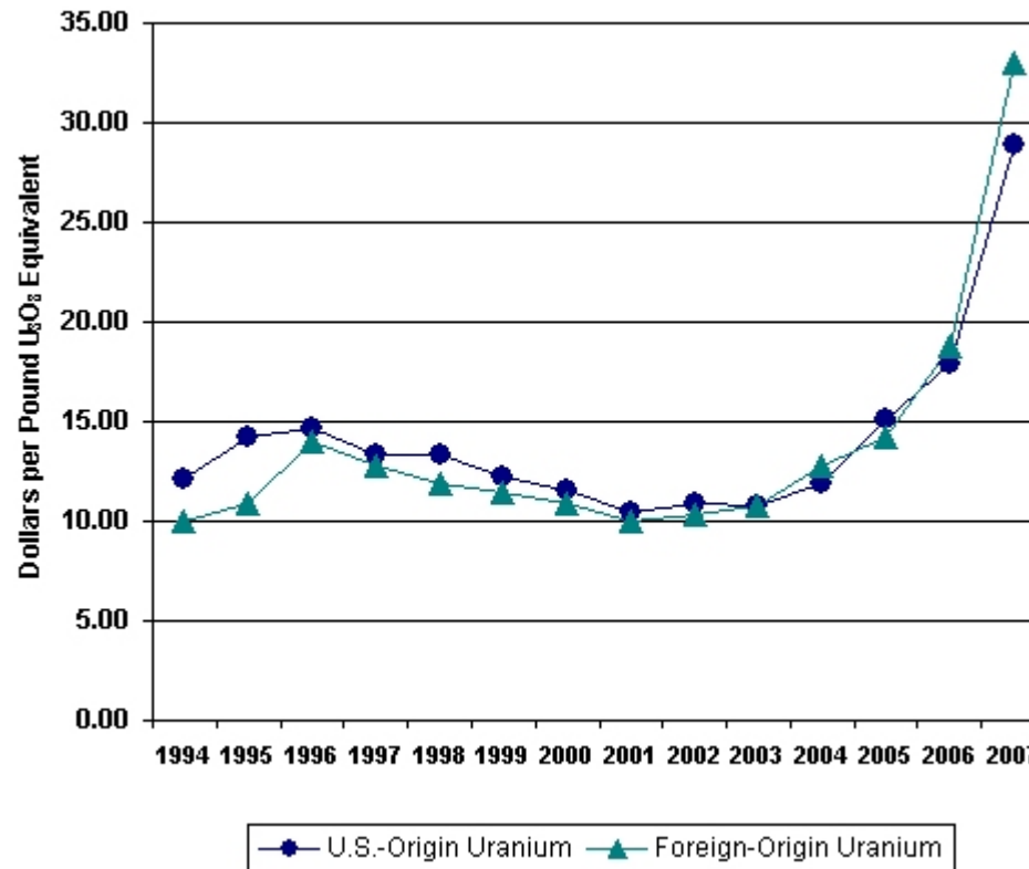
Figure S2. Weighted-Average Price of U.S. and Foreign-Origin Uranium Purchased by Owners and Operators of U.S. Civilian Nuclear Power Reactors, 1994-2007 Deliveries
