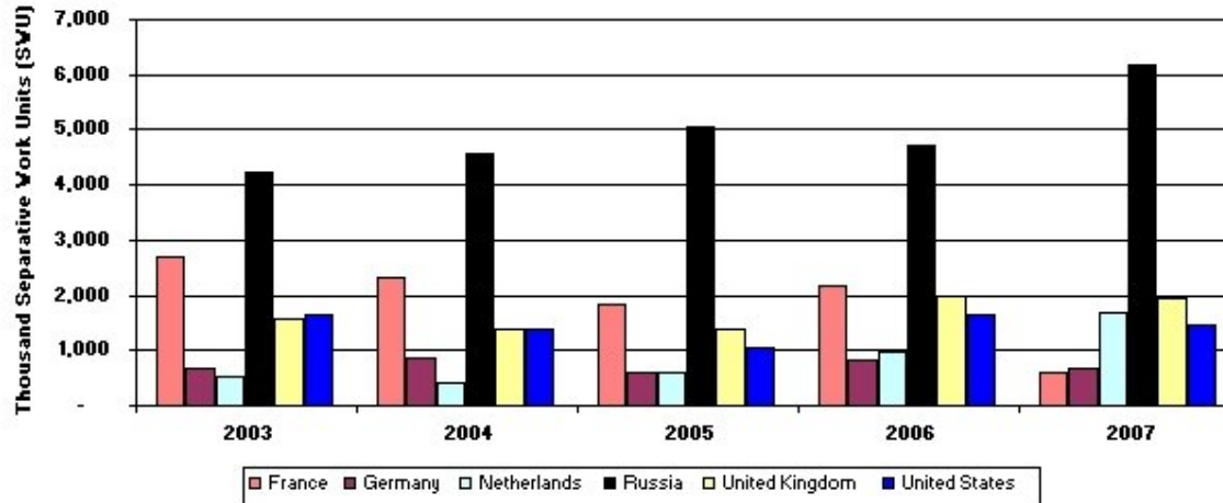
Figure 15. Purchases of Enrichment Services by Owners and Operators of U.S. Civilian Nuclear Power Reactors by Origin Country and Delivery Year, 2003-2007
