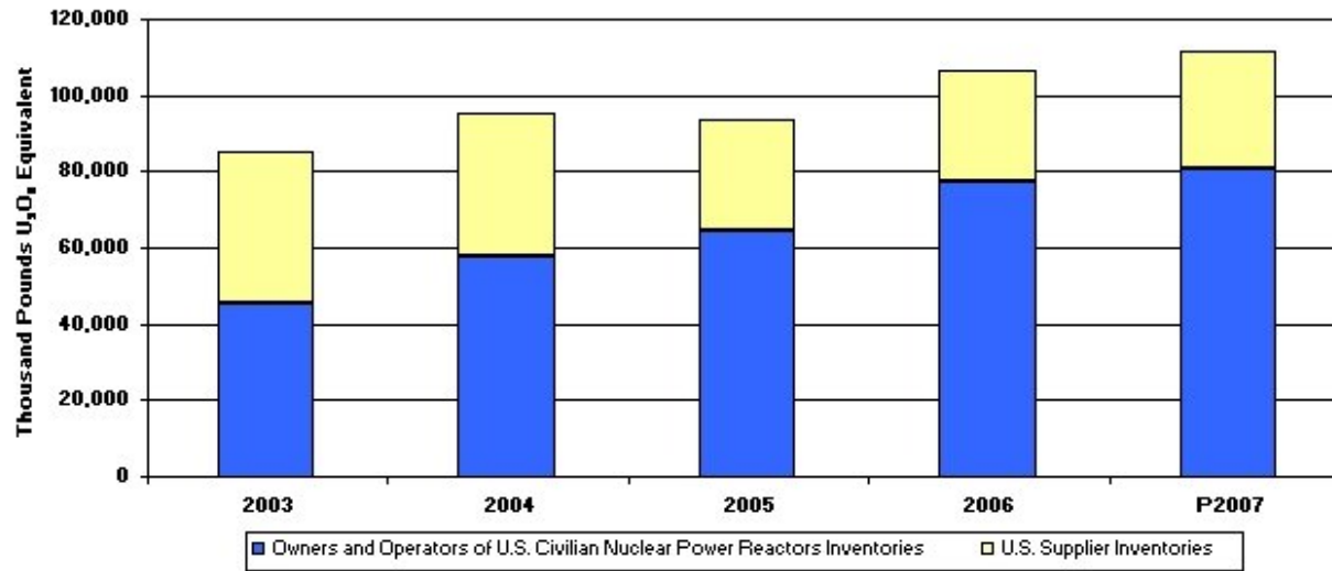
Figure 20. Commercial Inventories of Natural and Enriched Uranium as of End of Year, 2003-2007
