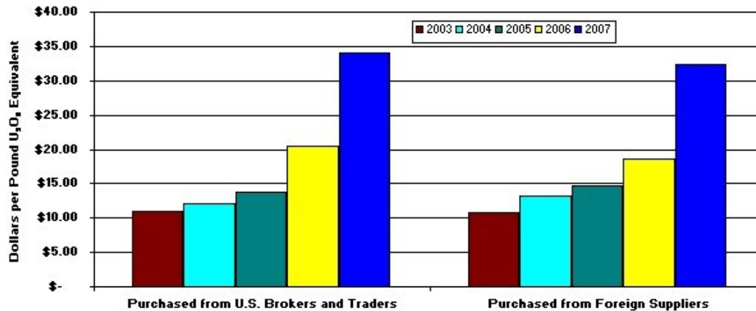
Figure 2. Weighted-Average Price of Uranium Purchased by Owners and Operators of U.S. Civilian Nuclear Power Reactors by Supplier and Delivery Year, 2003-2007
