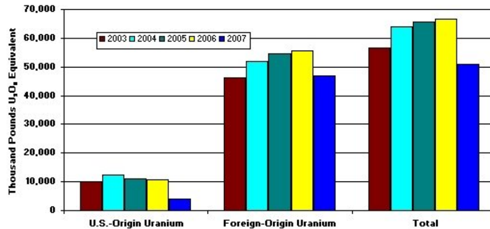
Figure 3. Uranium Purchased by Owners and Operators of U.S. Civilian Nuclear Power Reactors by Origin and Delivery Year, 2003-2007
