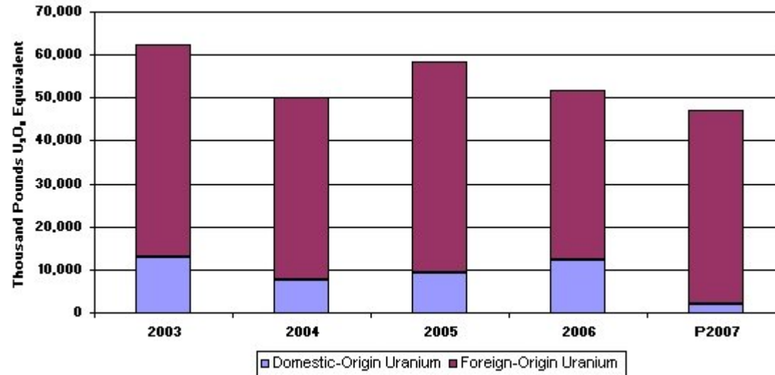
Figure 16. Uranium in Fuel Assemblies Loaded into U.S. Civilian Nuclear Power Reactors by Year, 2003-2007
