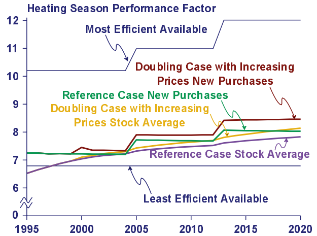
Figure 6. New Purchase and Stock Average Efficiencies of Heat Pumps, 1995-2020
