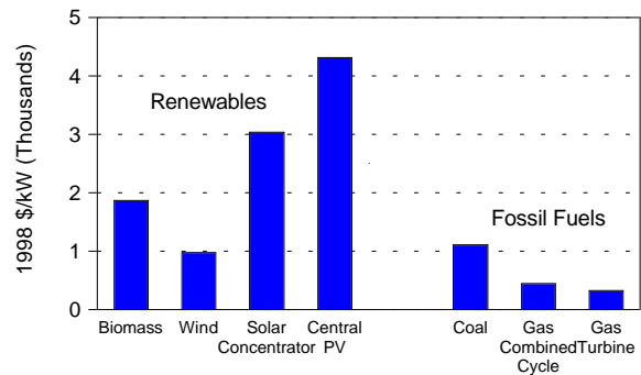
Figure 22. Capital Costs of Electric Generating Technologies
