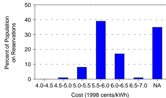
Figure 17. Distribution of Wind Development Costs Excluding Transmission Costs
