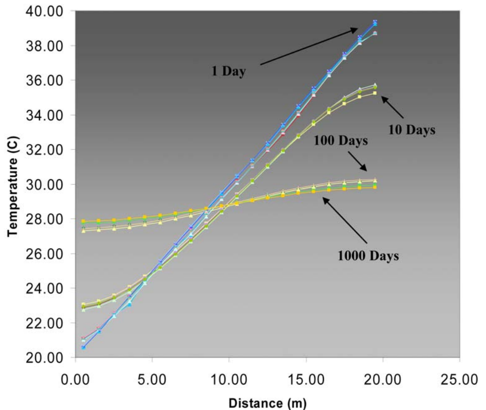
A comparison of model predictions of temperature distribution using HydrateResSim, MH2I HYDRES, CMG STARS, STOMP-HYD, and TOUGH-FX/Hydrate to test basic heat and mass transfer in the models. The temperature profiles have been plotted for each model as a separate trace for each of four times.
