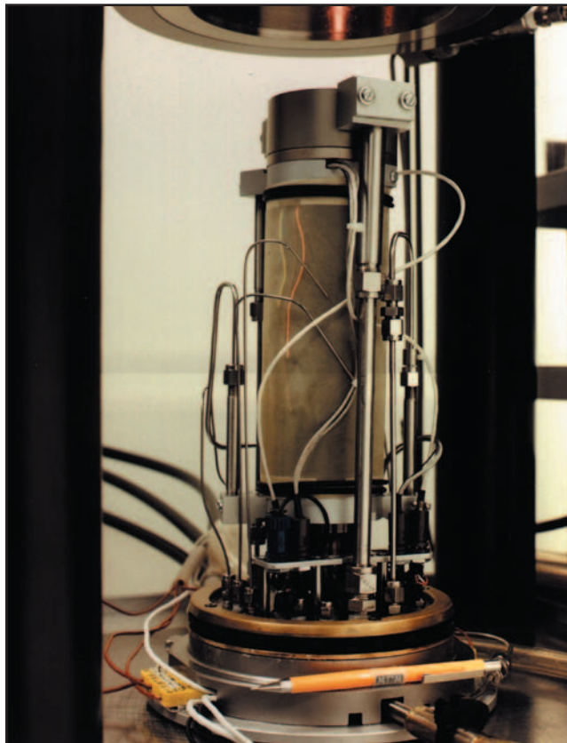
Close-up view of a test specimen about to be raised into the main pressure vessel (visible at the top of the photograph).
