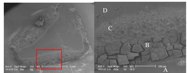
Figure 2 Corrosion beneath a crevice contact area.
