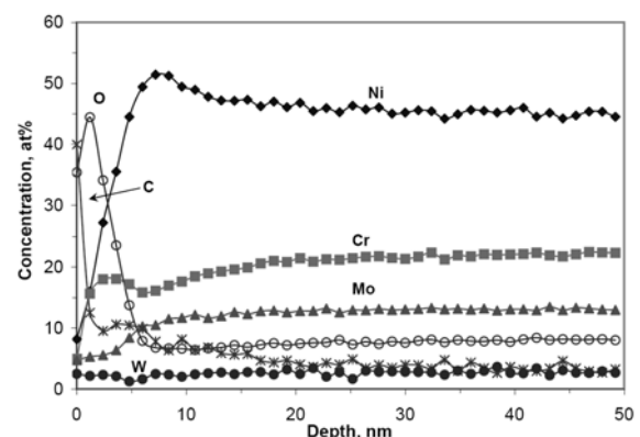
Figure 3 AES profiles on metal after 60 μm corrosion penetration in the creviced area
