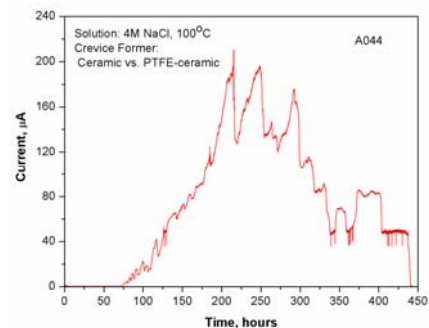
Figure 1 Polarization current with time during crevice test
