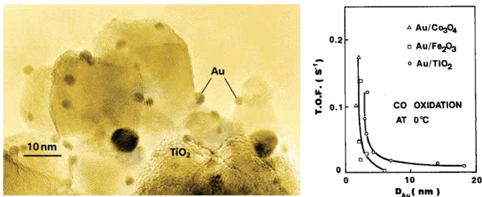
Figure 3.1. Transmission electron micrograph of gold (Au) nanoparticle catalysts on a titania ( TiO_2 ) support. The remarkable catalytic behavior of the gold nanoparticles for CO oxidation is shown on the right as a function of their size (© 1997 Elsevier; reprinted by permission [1]).
