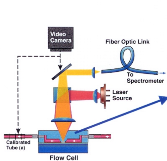
Fig. 2. Compact microfluidic system for reading nanolaser chip output spectra and images for high throughput analysis of endospores.
