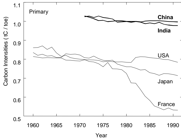
Figure 5.4: Carbon intensities of primary energy expressed in tons of carbon per ton of oil equivalent energy. Note that the zero of the carbon-intensity axis is suppressed. Source: Nakicenovic (1996).
