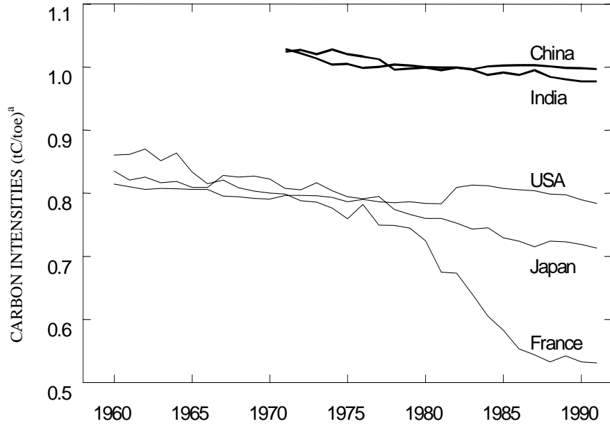
Figure E.13: Carbon intensities of primary energy expressed in tons of carbon (tC) per ton of oil equivalent energy (toe).
