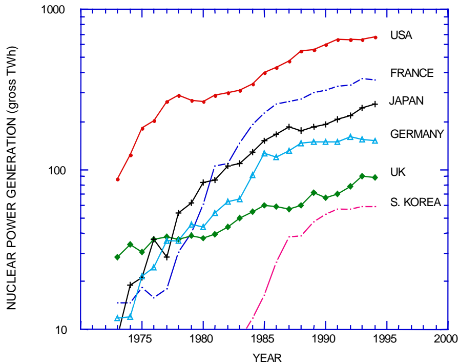
Figure E.1: Growth of annual nuclear power generation in selected countries, 1973-1994.
