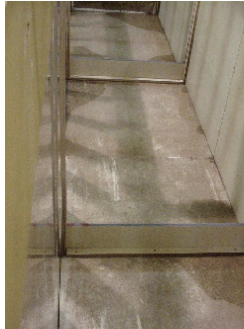
Figure 19 - View of 6 inch high weirs used to induce large scale vertical oriented eddies in the flow along the invert of the test flume.
