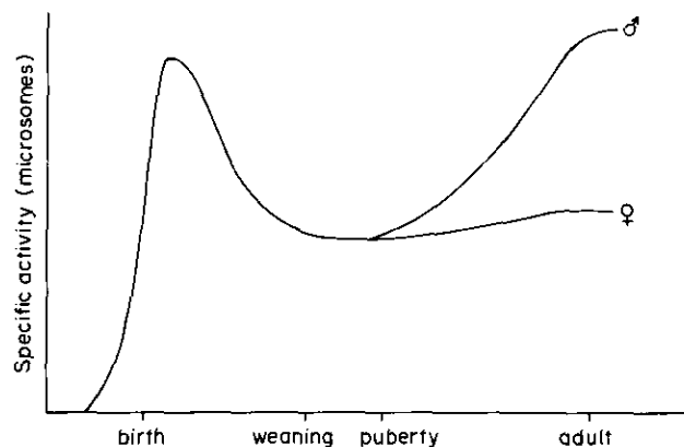
FIGURE 4. Schematic representation of glucuronidation rates of one group of substrates by UDP glucuronyltransferase. This scheme was derived as a composite of several studies (10, 33, 38, 39).
