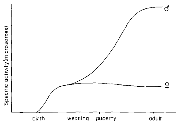
FIGURE 2. Schematic representation of aryl hydrocarbon hydroxylase ontogeny in rat liver. This scheme was derived as a composite of many studies (10, 16, 21, and unpublished observations).
