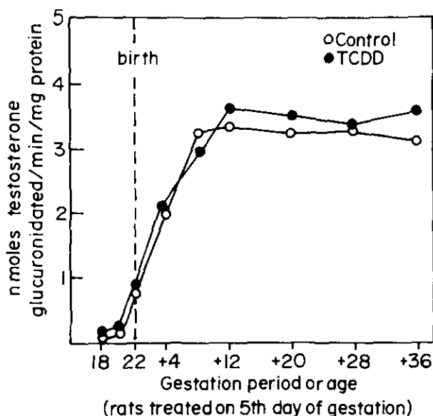
FIGURE 7. Effects of treatment of pregnant rats with 3 \mu g TCDD/kg on the ontogeny of hepatic testosterone glucuronidation activity. Each value derived from at least four separate litters. Assay methods presented elsewhere (38).
