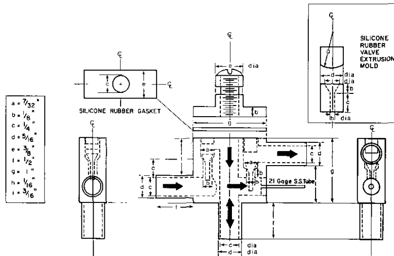
FIGURE 5. Tracheal valve system. Inset is a diagram of the silicone rubber valve extrusion mold.
