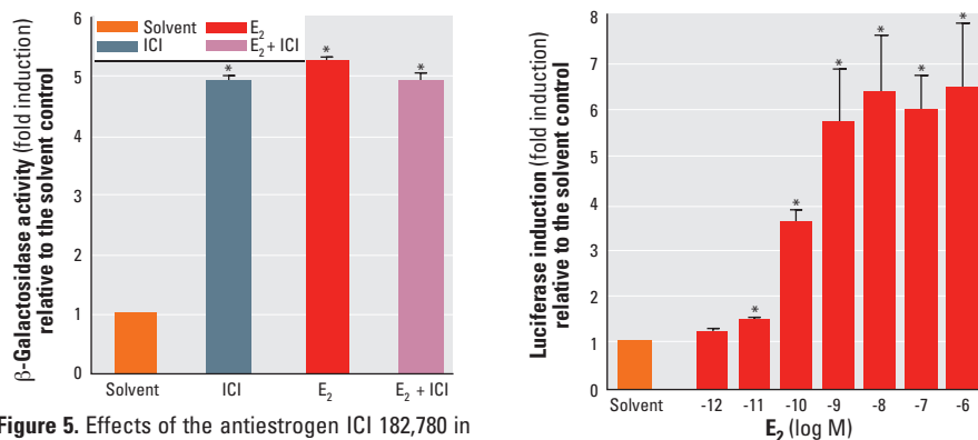
Figure 6. Induction of luciferase activity in MCF-7 cells by E 2 . MCF-7 cells at 80% confluency and stably transfected with the reporter plasmid ERE-luc were treated with increasing concentrations of E 2 . Data are presented as mean \pm SD and represent three independent experiments representing six measurements.
