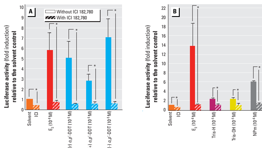
Figure 8. Inhibition of environmental chemical-induced luciferase activity by the antiestrogen ICI 182,780. MCF-7 cells stably transfected with pERE-luc were treated with vehicle, E 2 , or environmental chemicals in the presence or absence of 10 -6 M ICI 182,780. Data are presented as mean \pm SD and represent three independent experiments representing six measurements. * p < 0.05.
