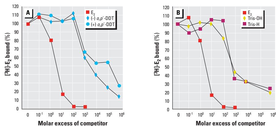
Figure 2. Inhibition of [^3\text{H}]\text{-E}_2 binding by environmental chemicals. Some compounds tested in the CARLA assay were measured for their ability to inhibit the binding of [^3\text{H}]\text{-E}_2 to hER by displacing it in competition binding assays. MCF-7 cells growing in monolayer culture were incubated with 0.1 nM [^3\text{H}]\text{-E}_2 for 1 hr at 37^\circ\text{C} in the absence or presence of increasing concentrations of radioinert E_2 , (-) o,p' -DDT, (+) o,p' -DDT, Tris-H, or Tris-OH. The data are plotted as the percentage of control in which specific binding in the absence of competitor is equal to 100%.
