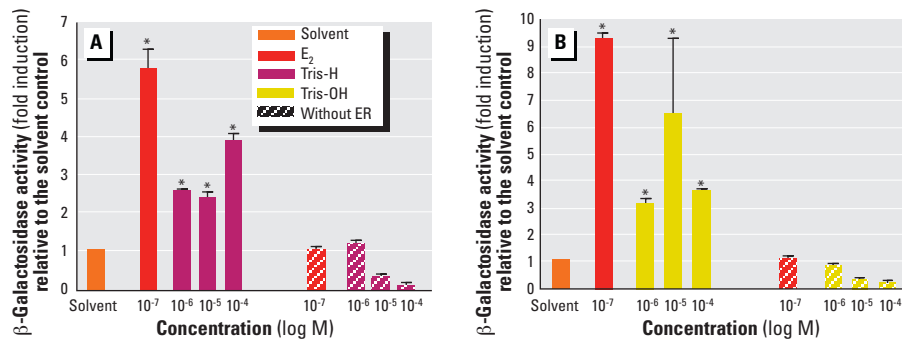
Figure 4. Response of YRG-2 yeast cells, which contain the reporter plasmid pLGERE and that express or do not express hER, to Tris-H (A) and Tris-OH (B). Following overnight incubation the cultures were assayed for the \beta -galactosidase activity (see “Materials and Methods” for details). Values represent the \beta -galactosidase induction relative to the solvent control. Values are mean \pm SD of at least two independent experiments in triplicate.
