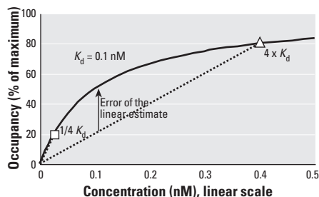
Figure 3. Error in predicting actual receptor occupancy based on linear estimation applied to a saturating test dose. Receptor occupancy (solid line) is graphed against a linear scale of ligand concentration from 0 to 0.5 nM, where the K_d for ligand binding = 0.1 nM. Linear estimations to zero concentration (dotted lines) are shown originating from single measurements at two test doses, one below the K_d (square point of origin, at 1/4 K_d = 0.025 nM) and one above the K_d (round point of origin, at 4 \times K_d = 0.4 nM). This assumes no background-contaminating estrogenic activity from either endogenous or exogenous sources other than the chemical being tested. Where the test dose used as the origin of the linear estimation is below the K_d , the linear estimation is very close to actual occupancy. Where the lowest test dose used as the origin of the linear estimation to zero dose is above the K_d , the linear estimation deviates substantially from actual receptor occupancy, indicated as “Error of the linear estimate.” The fold-underestimate of occupancy, and therefore underestimate of response for receptor-mediated events, increases as the origin of measurement increases above the K_d and is calculated in Table 2 for a number of EEDCs where the origin is 10,000-fold above the K_d , which could not be shown to scale on this figure.
