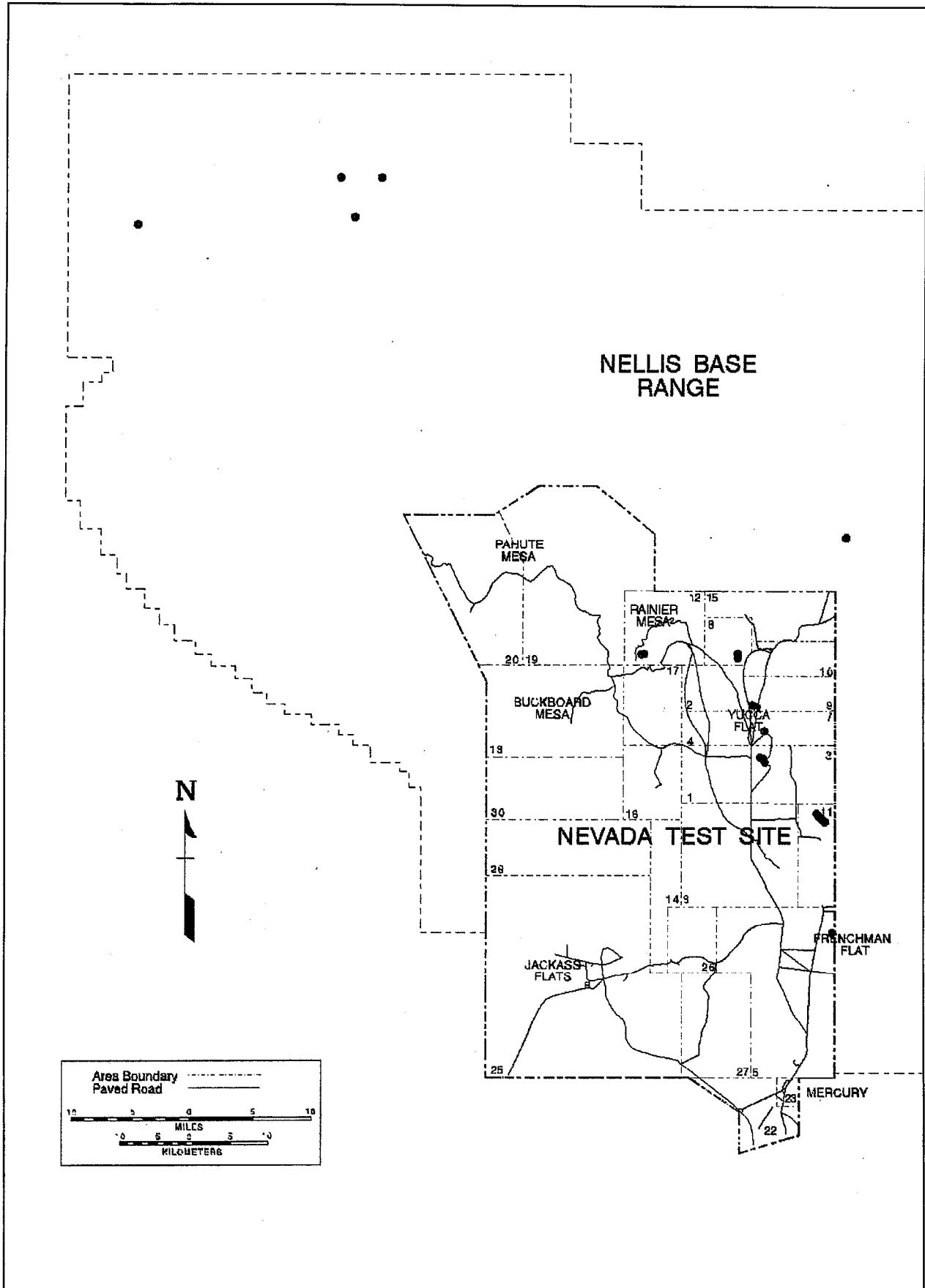
Figure 2.3 Location of Safety Tests on NTS and the Nellis Base Range
