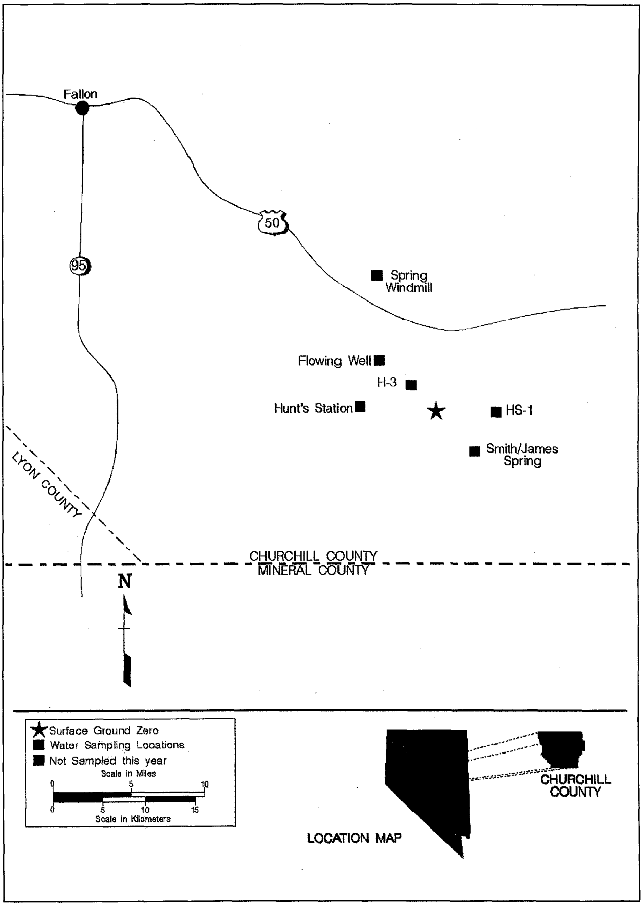
Figure 9.6 LTHMP Sampling Locations for Project SHOAL - 1995
