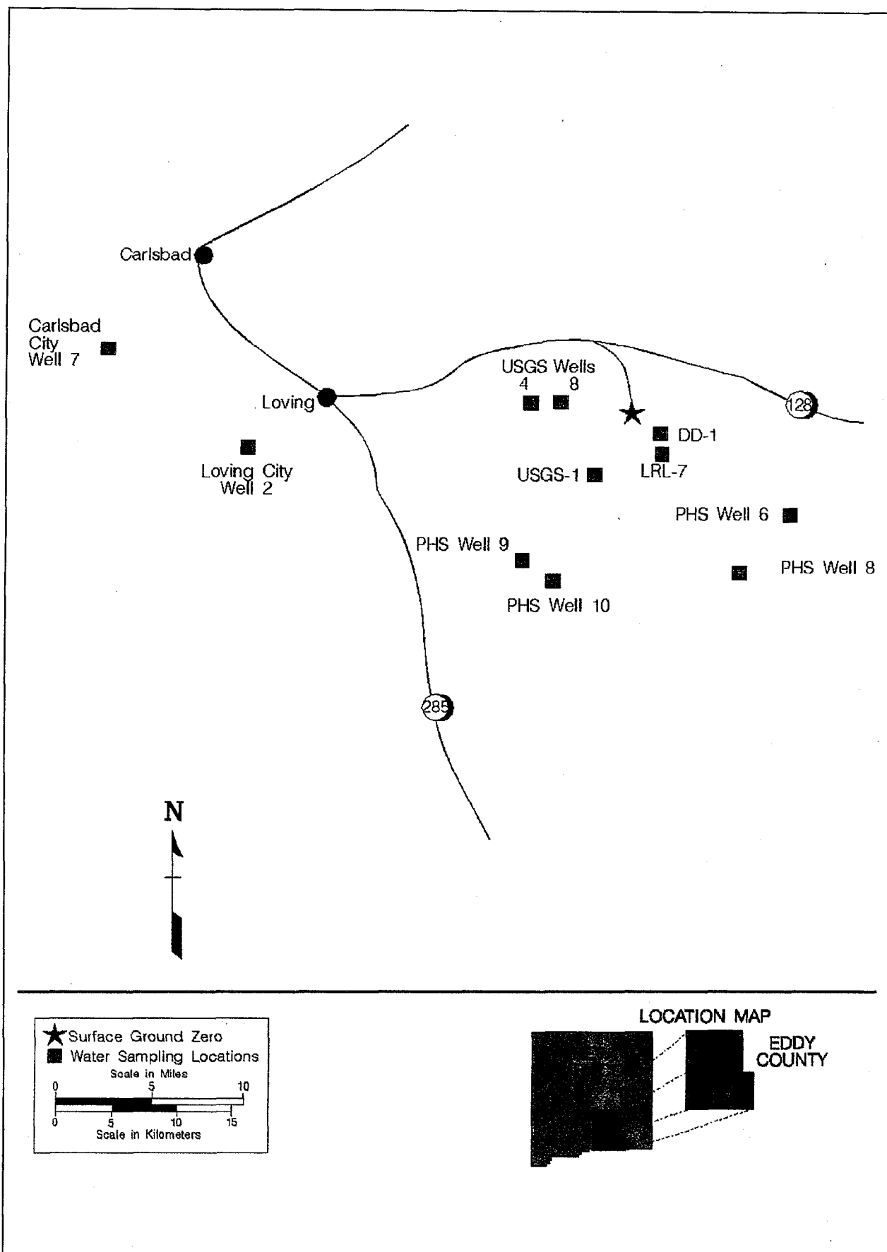
Figure 9.10 LTHMP Sampling Locations for Project GNOME - 1995
