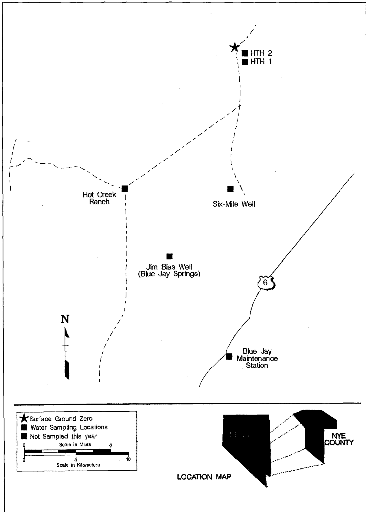
Figure 9.5 LTHMP Sampling Locations for Project FAULTLESS - 1995
