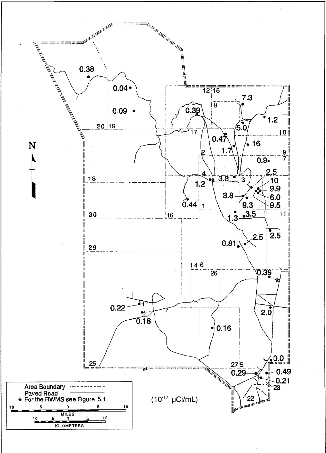
Figure 5.4 NTS Airborne ^{239+240}\text{Pu} Annual Average Results - 1995
