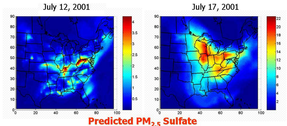
CTM results for regional \text{PM}_{2.5} "episode" in July 2001
