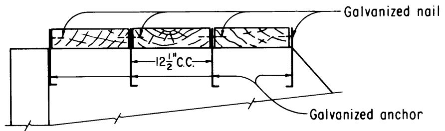
END VIEW
