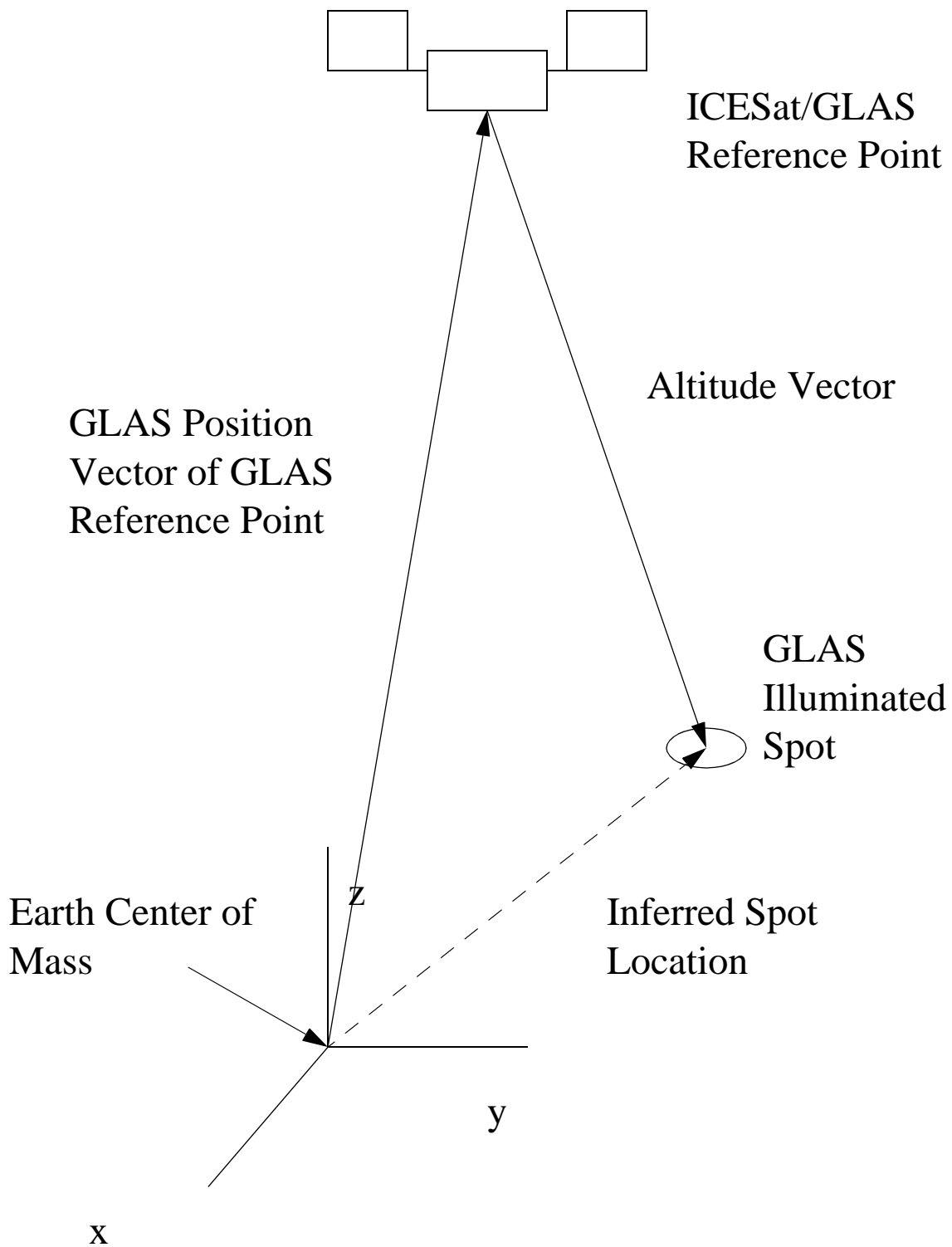
Fig. 1. Altimetry Concept
