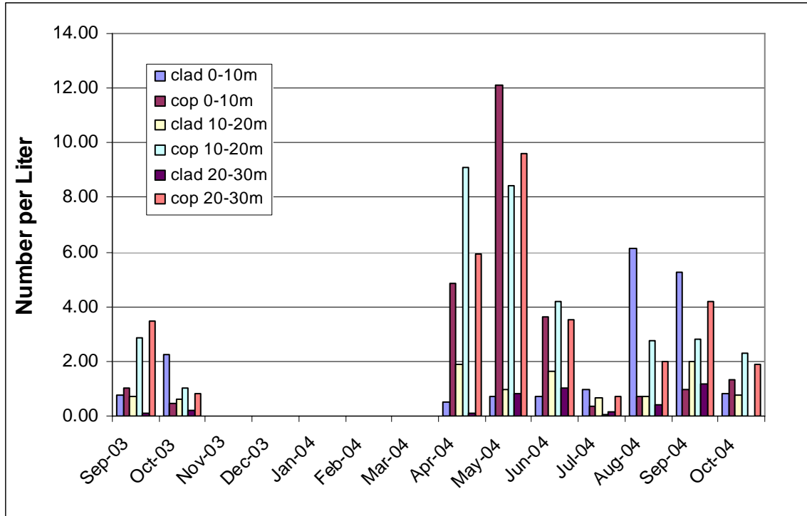
Figure 3. Seasonal abundance and distribution of cladoceran and copepod zooplankton in three depth strata at Cle Elum station CLE2 from September 2003 to October 2004.
