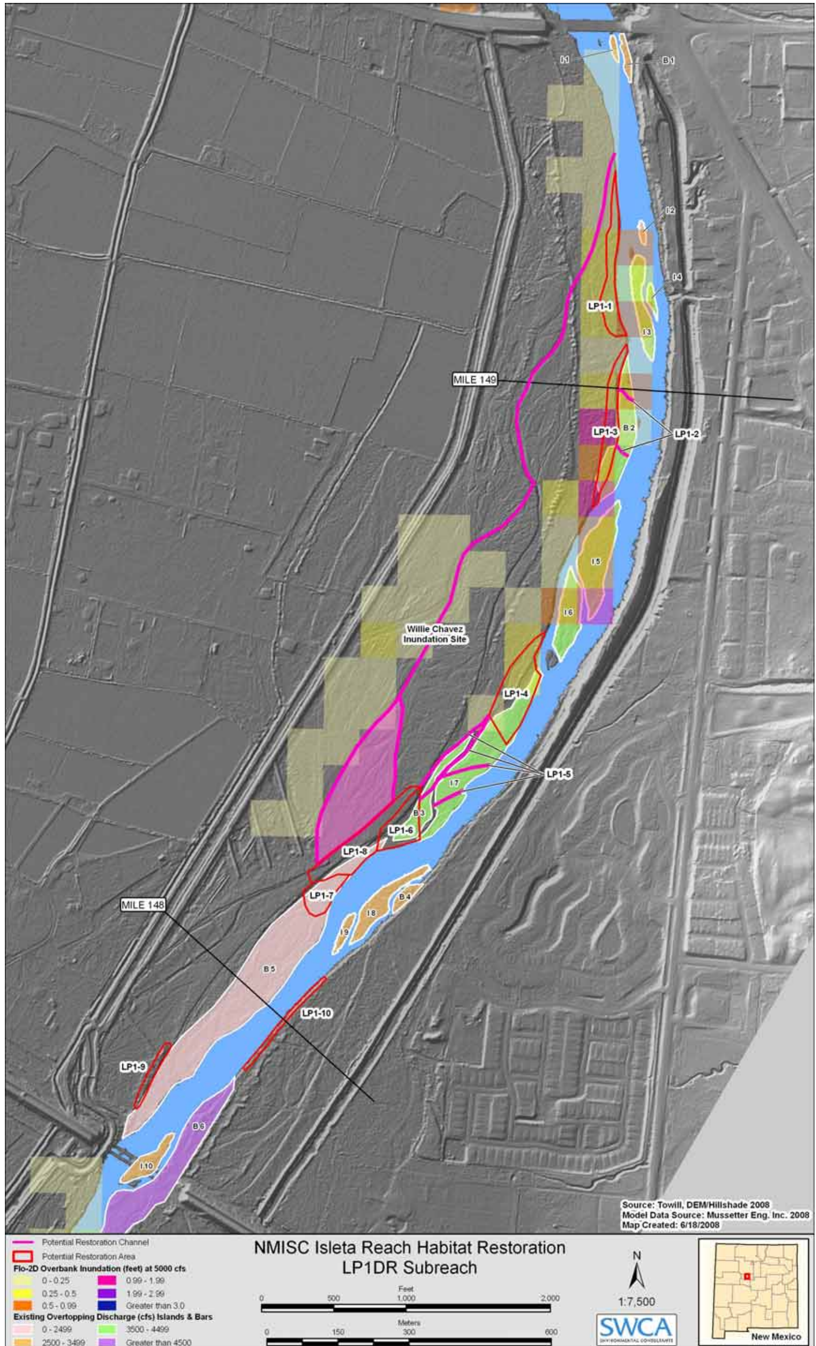
Figure B.4. LP1DR Subreach with Bosque inundation site FLO-2D modeling with island/bar and restoration site delineation displayed on the DEM.
