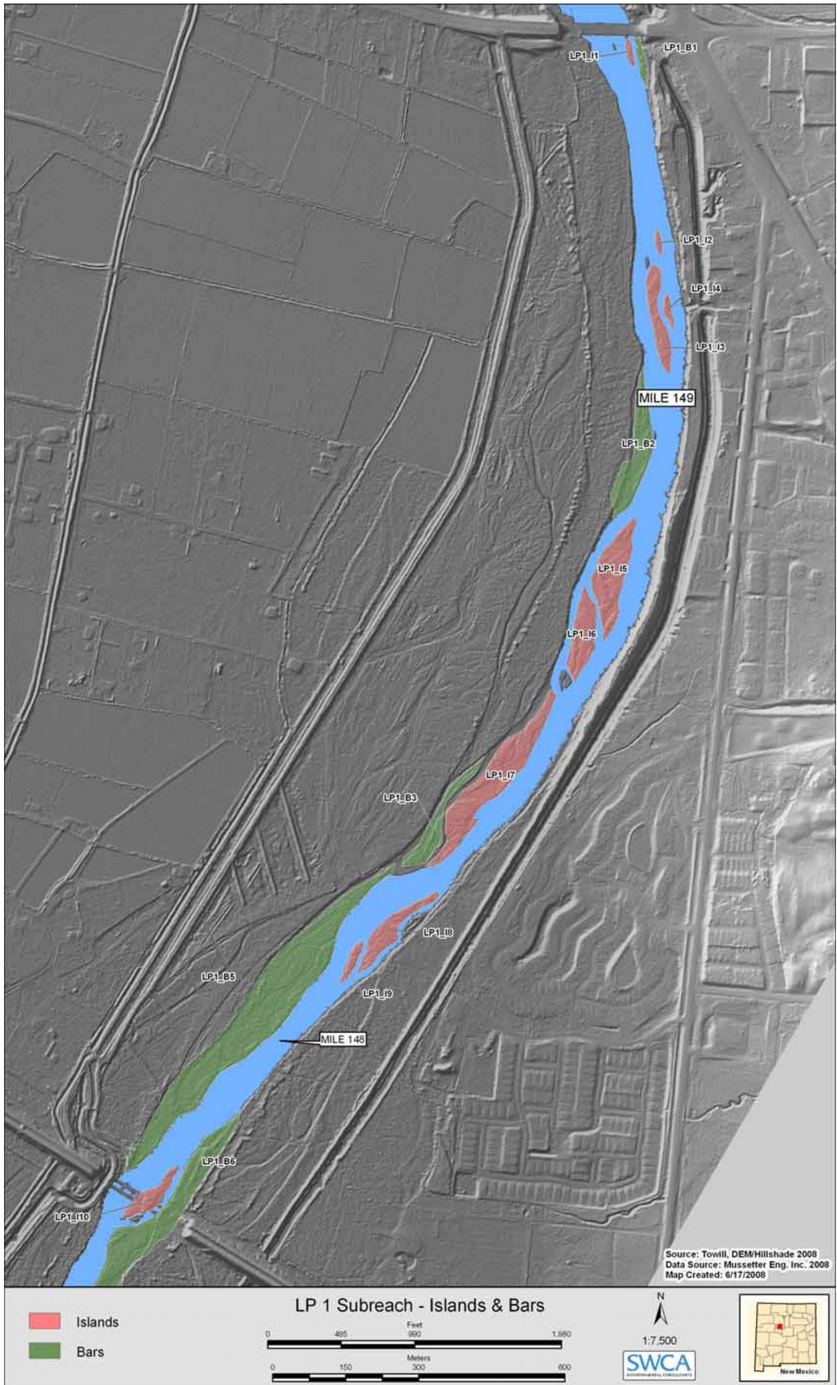
Figure B.6. LP1DR Subreach with Bosque inundation site island and bar delineation displayed on the (DEM).
