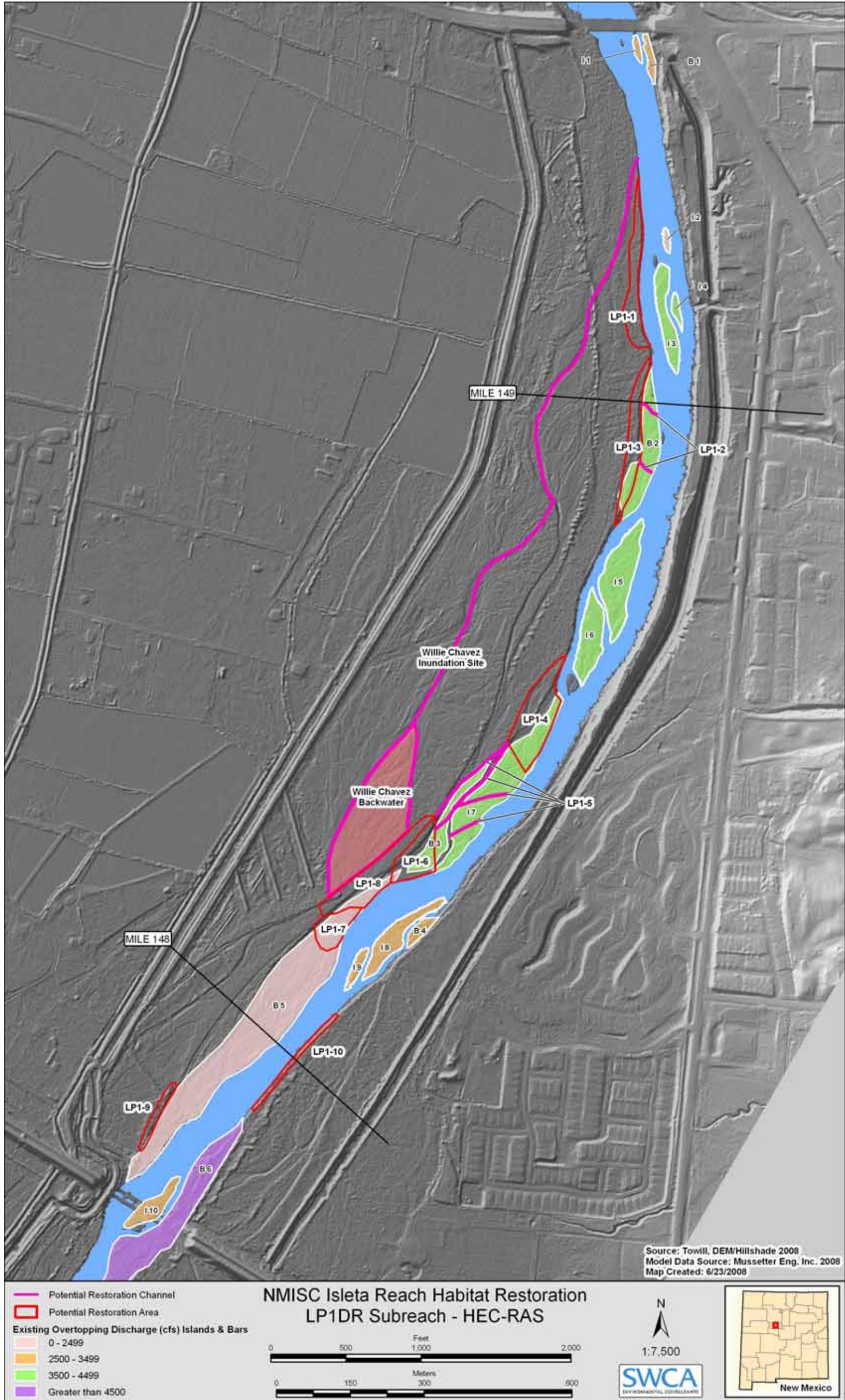
Figure B.5. LP1DR Subreach with Bosque inundation site HEC-RAS modeling with island/bar and restoration site delineation displayed on the DEM.
