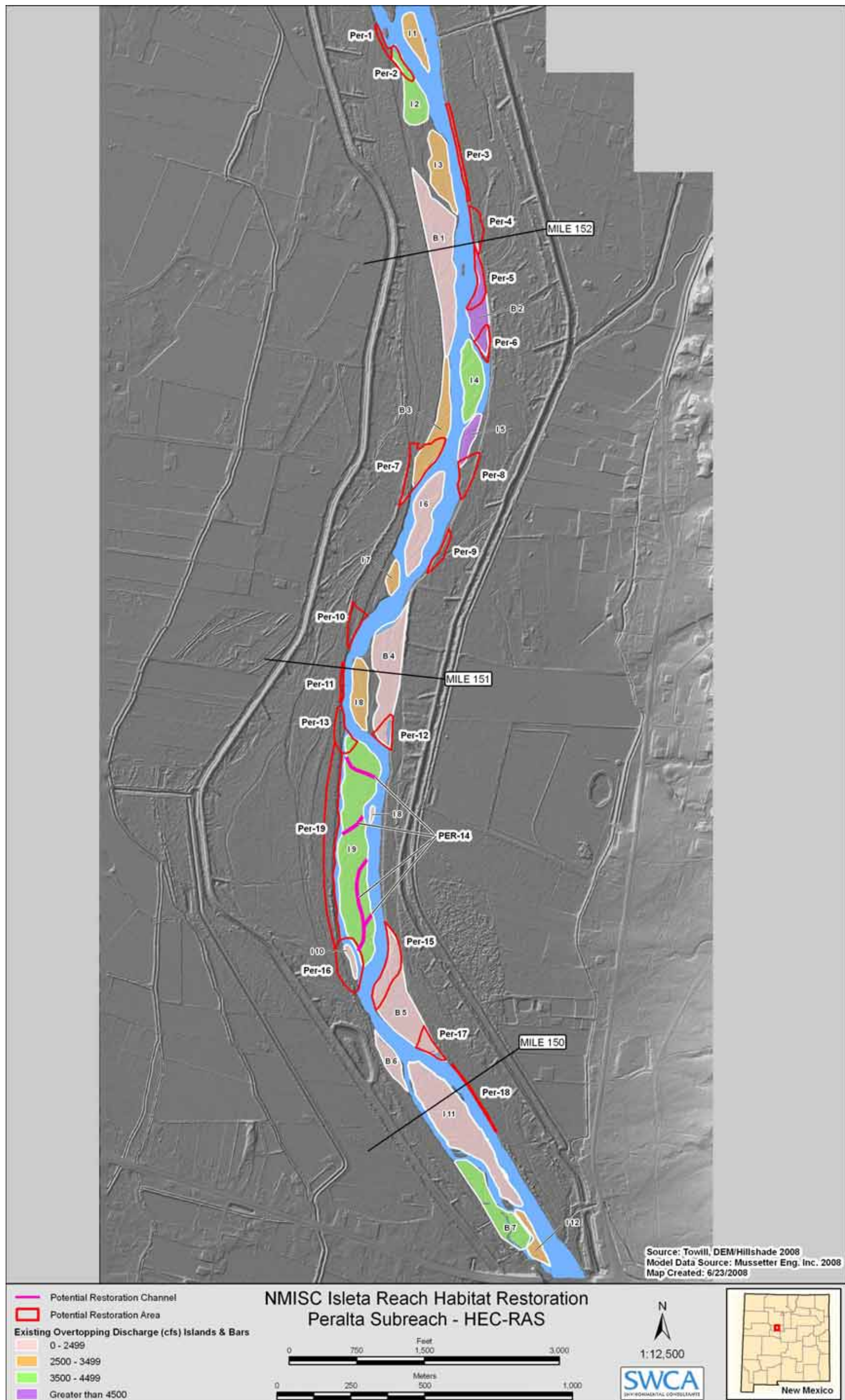
Figure B.2. Peralta Subreach HEC-RAS modeling with island/bar and restoration site delineation displayed on the DEM.
