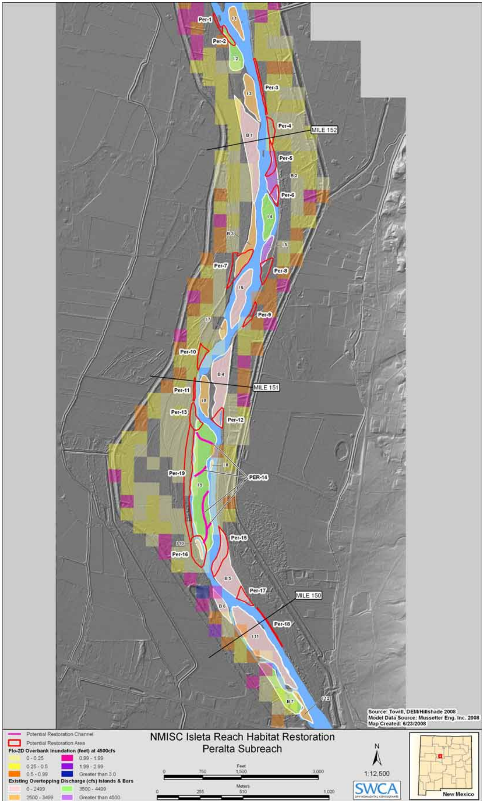
Figure B.1. Peralta Subreach FLO-2D modeling with island/bar and restoration site delineation displayed on the digital elevation model (DEM).
