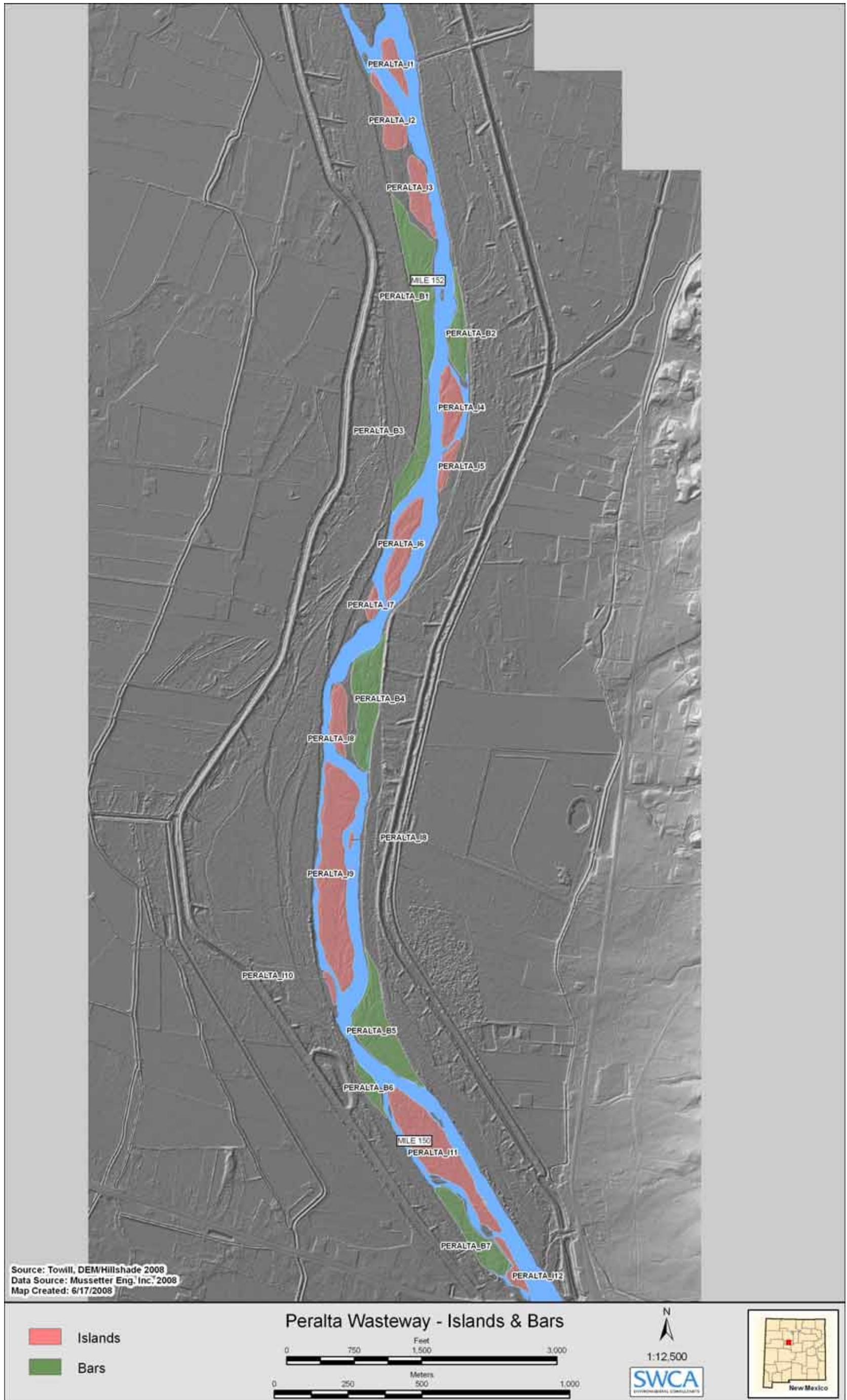
Figure B.3. Peralta Subreach island and bar delineation displayed on the DEM.
