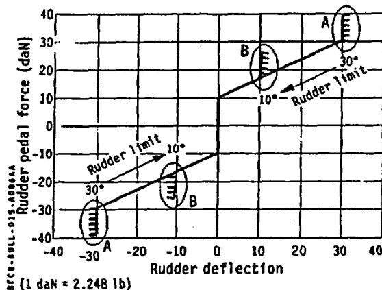
A310/A300-600 Rudder feel system
