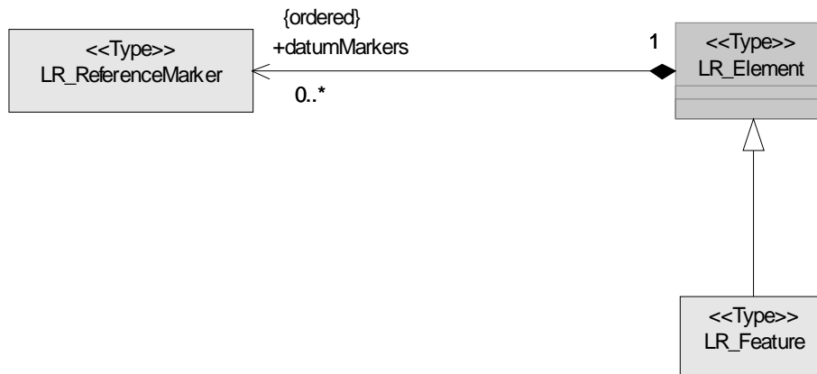
Figure B.7 – LR_Element
