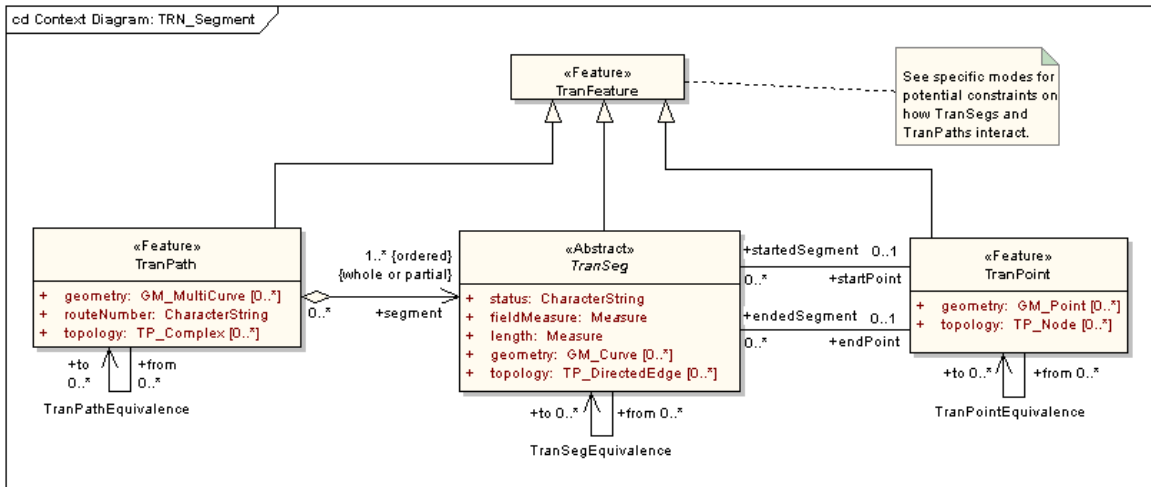
Figure 3 – Relationships among TranSeg, TranPoint, and TranPath
