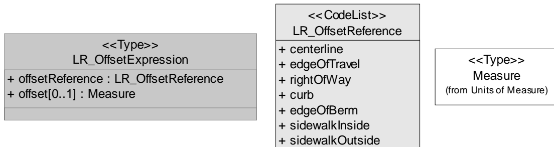
Figure B.8 – LR_OffsetExpression
