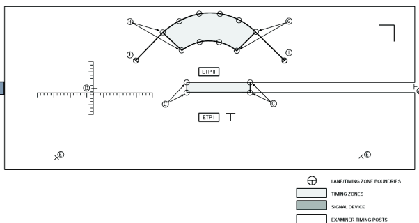
MOTORCYCLIST LICENSING SKILL TEST COURSE LAYOUT
