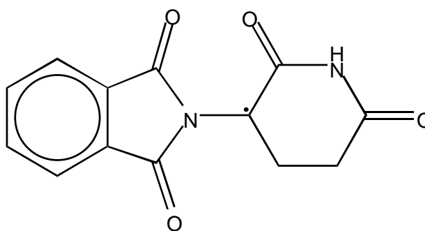
Chemical Structure of thalidomide
