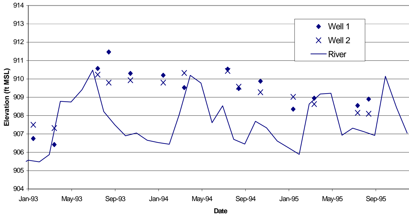
FIGURE 2.2-3 MONTHLY AVERAGE ON-SITE WELL ELEVATIONS AND RIVER ELEVATIONS, 1993-1995
