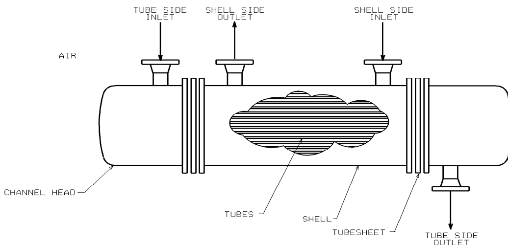
Figure C2.2-1 Simplified Shell-and-Tube Heat Exchanger
