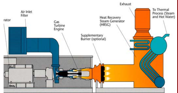
Components of typical gas-fired turbine CHP unit
