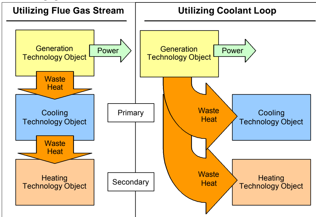
Figure 4 BCHP Utilization of Thermal Energy
