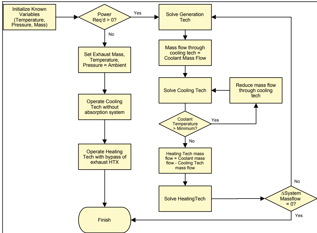
Figure 8 BCHP Solution Utilizing Coolant Loop
