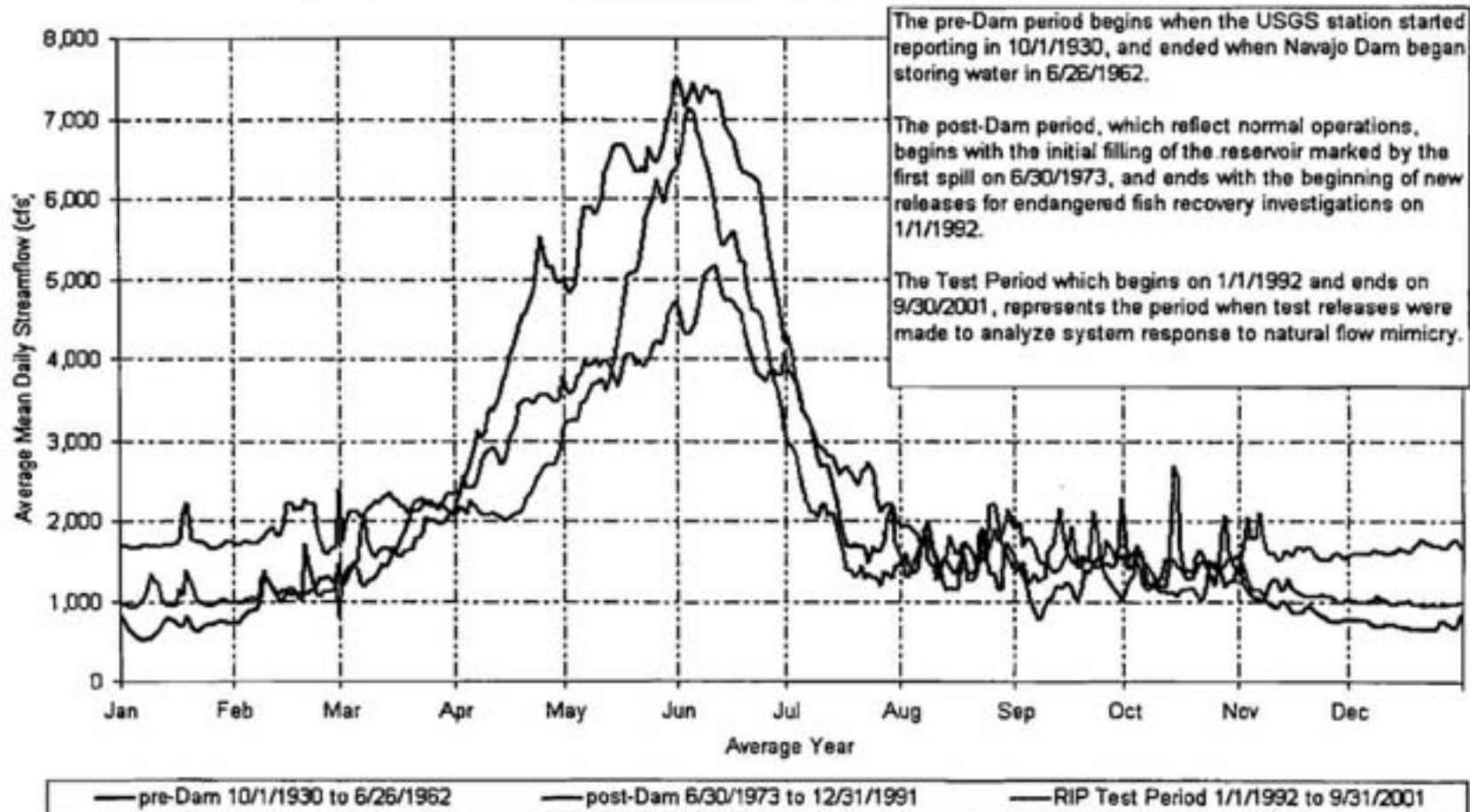
Figure 2. . Graph comparing pre-Navajo Dam, post-Navajo Dam (pre-Flow Recommendations), and proposed action flow of San Juan River past the Bluff gage.
