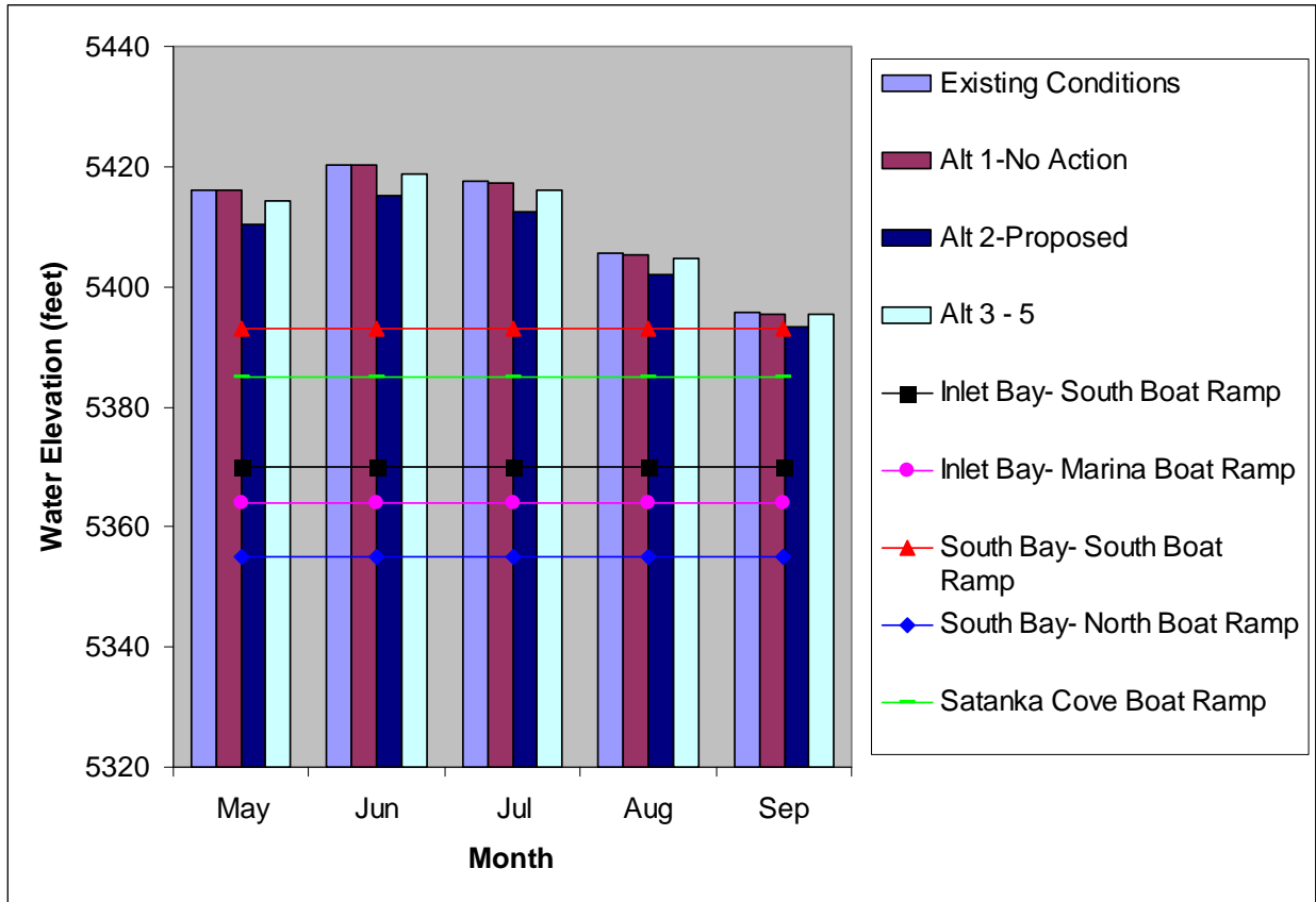
Figure 20. Average Monthly Water Levels at Horsetooth Reservoir Boat Ramps under Cumulative Effects.
