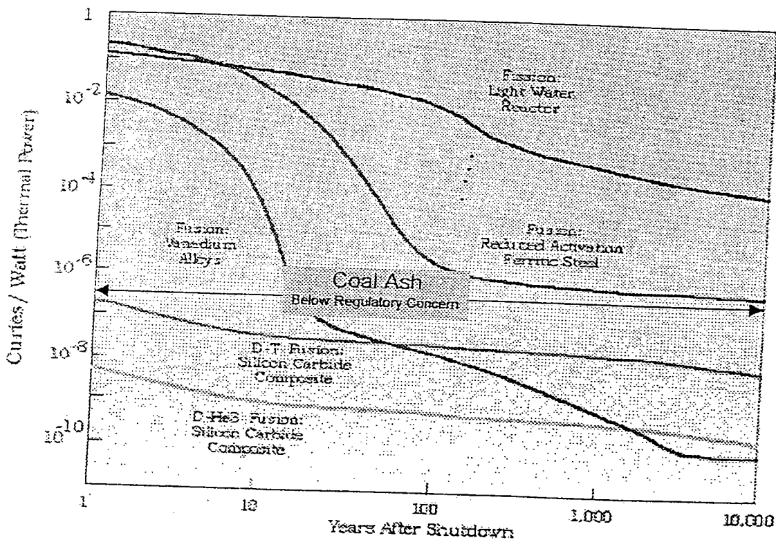
Figure 2: Radioactive byproducts from fusion and fission. Fusion byproducts for structural materials under development are relatively short-lived, becoming comparable in radioactivity to the equivalent coal ash in about one human lifetime or less. Coal ash radioactivity is considered to be below regulatory concern.
