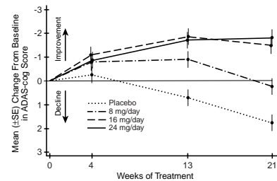
Figure 1: Time-Course of the Change From Baseline in ADAS-cog Score for Patients Completing 21 Weeks (5 Months) of Treatment
