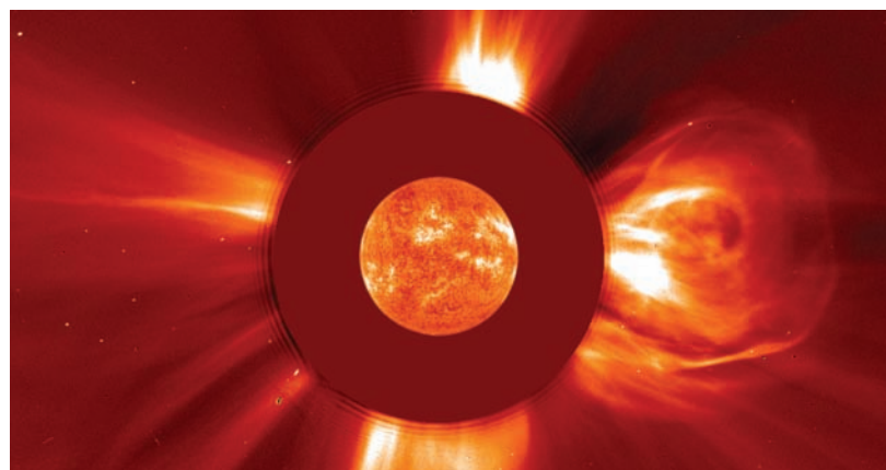
One of the largest solar flares ever recorded occurred at 4:51 p.m. EDT, on Monday, April 2, 2001, as observed by the Solar and Heliospheric Observatory (SOHO) satellite.
