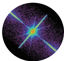
An X-ray image of black hole candidate XTE J1118+480.
